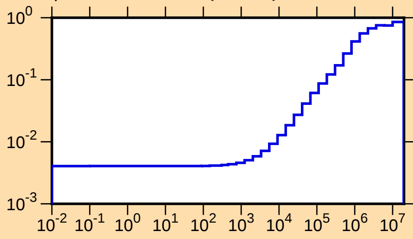
\mu vs. E for ^{175}\text{Re}(\text{mt251})
