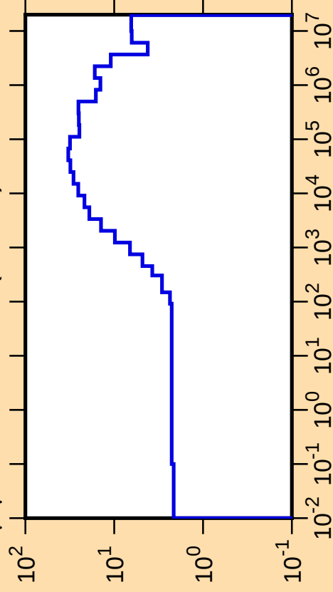
\Delta\mu/\mu vs. E for ^{175}\text{Re}(\text{mt251})
