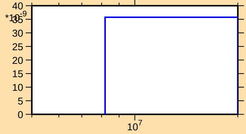
\sigma vs. E for ^{175}\text{Re}(\text{mt } 45)
