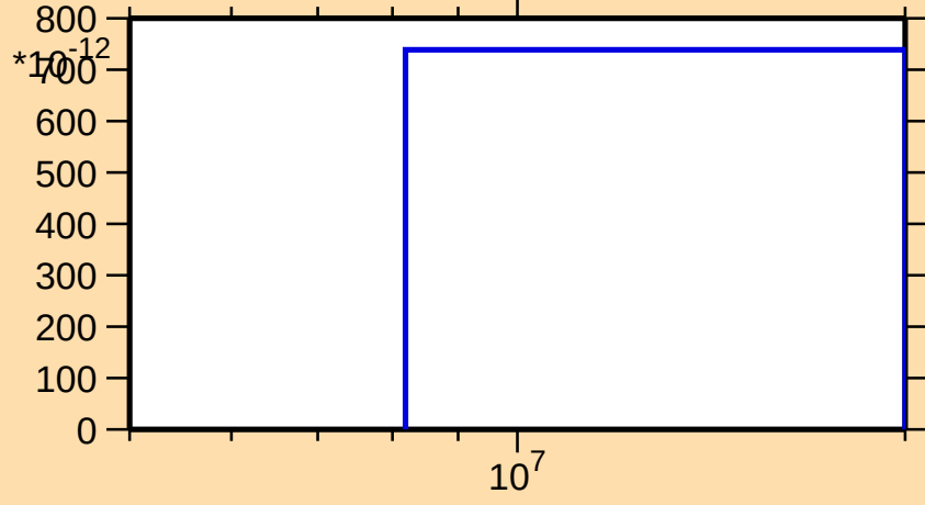
\sigma vs. E for ^{175}\text{Re}(\text{mt117})
