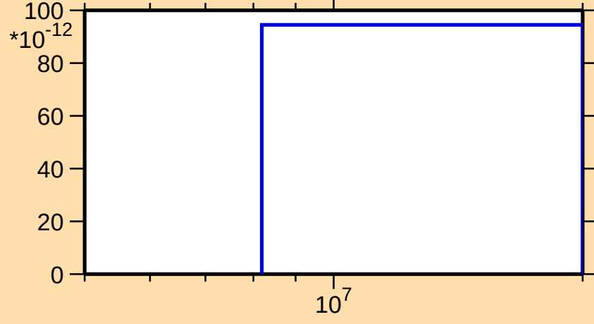
\sigma vs. E for ^{175}\text{Re}(n,\text{pd})
