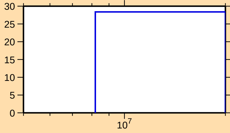
\Delta\sigma/\sigma vs. E for ^{175}\text{Re}(n,\text{inel.})
