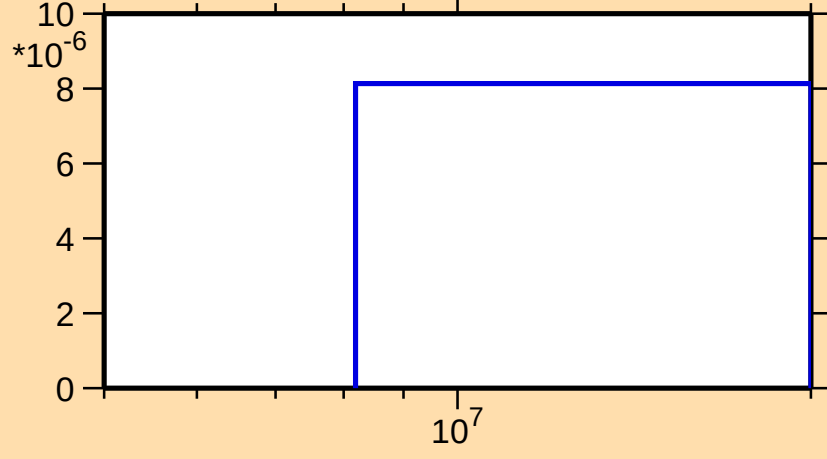
\sigma vs. E for ^{175}\text{Re}(n,3n)
