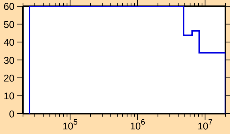
\Delta\sigma/\sigma vs. E for ^{175}\text{Re}(n,n_1)
