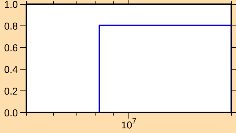
\sigma vs. E for ^{175}\text{Re}(n,2n)
