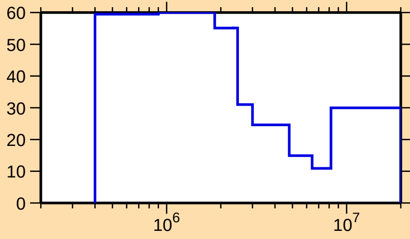
\Delta\sigma/\sigma vs. E for ^{175}\text{Re}(n,n\text{cont.})
