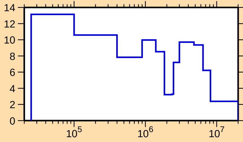
\Delta\sigma/\sigma vs. E for ^{175}\text{Re}(n,\text{tot.})
