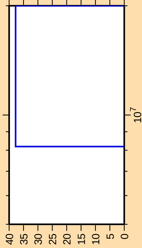
\Delta\sigma/\sigma vs. E for ^{175}\text{Re}(n,p)
