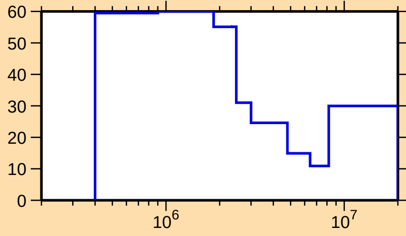
\Delta\sigma/\sigma vs. E for ^{175}\text{Re}(n,n\text{cont.})
