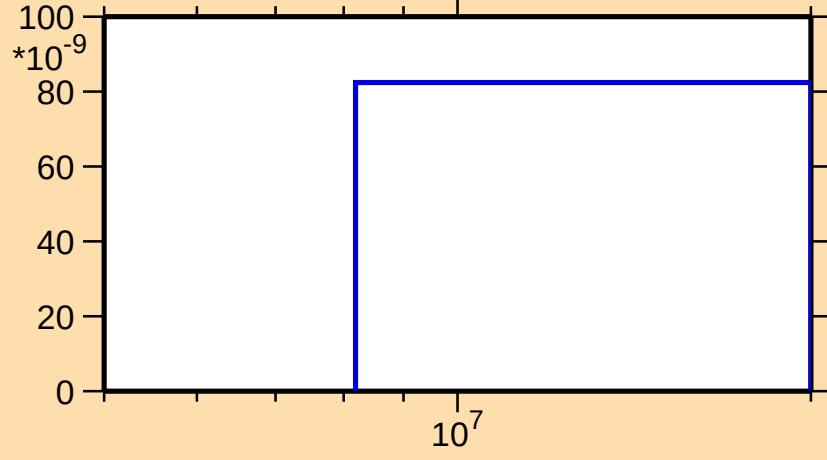
\sigma vs. E for ^{175}\text{Re}(n,2n\alpha)
