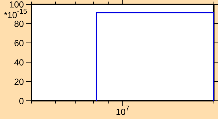
\sigma vs. E for ^{175}\text{Re}(n,\text{pt})
