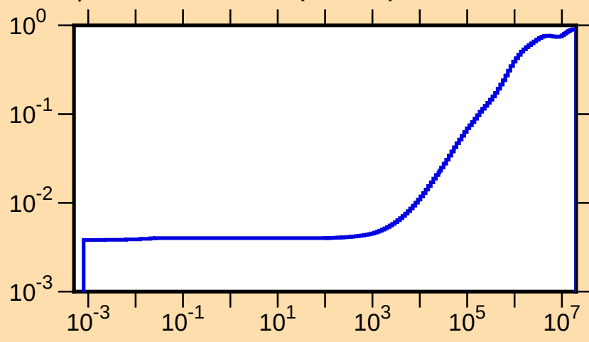
\mu vs. E for ^{177}\text{Re}(\text{mt251})
