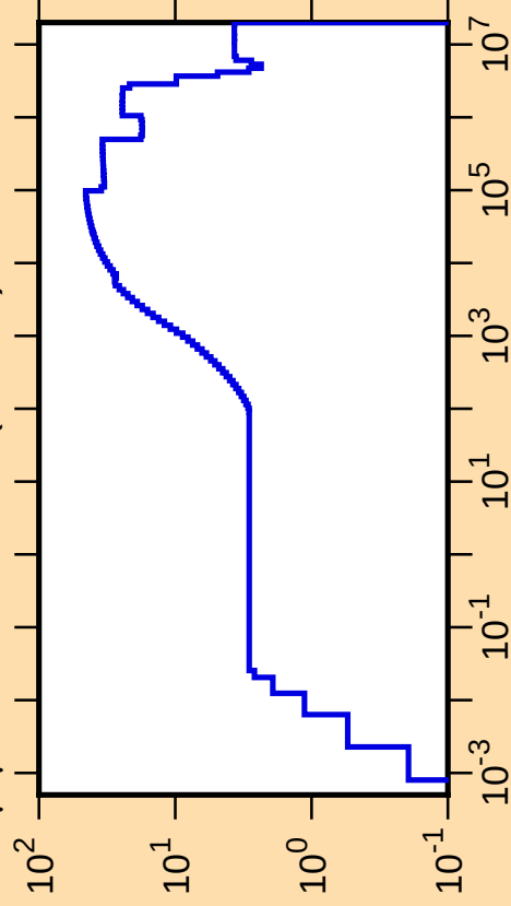
\Delta\mu/\mu vs. E for ^{177}\text{Re}(\text{mt251})
