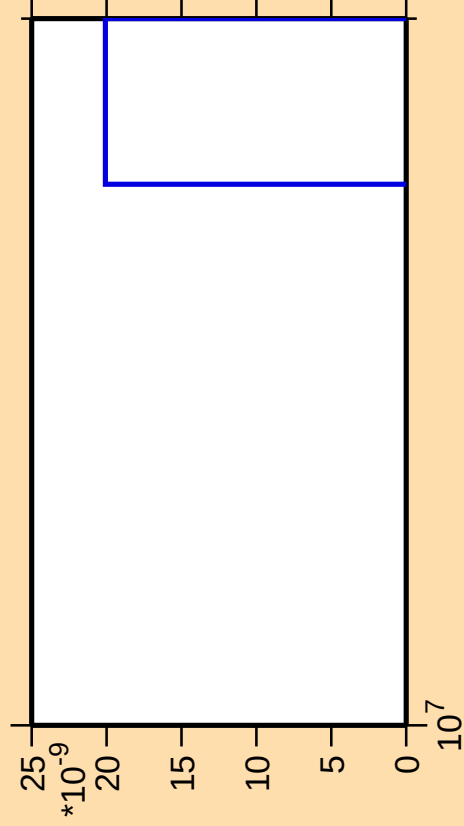
\Delta\sigma/\sigma vs. E for ^{177}\text{Re}(\text{mt } 42)
