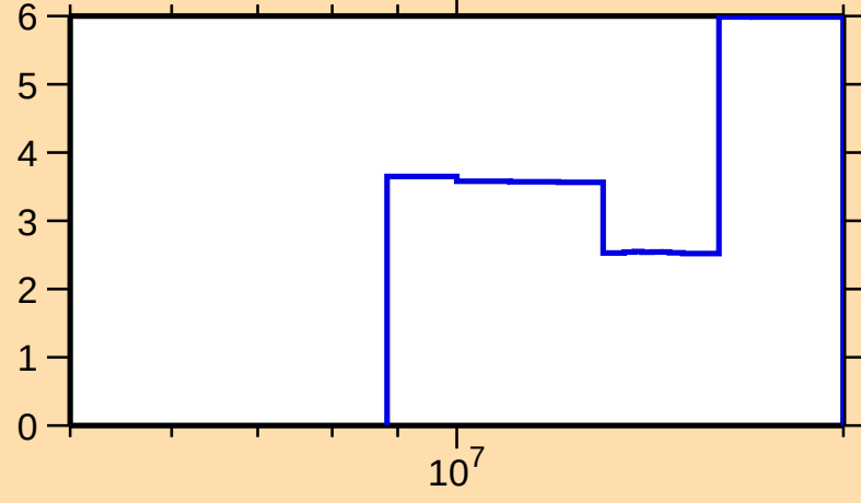
\Delta\sigma/\sigma vs. E for ^{177}\text{Re}(n,\text{el.})
