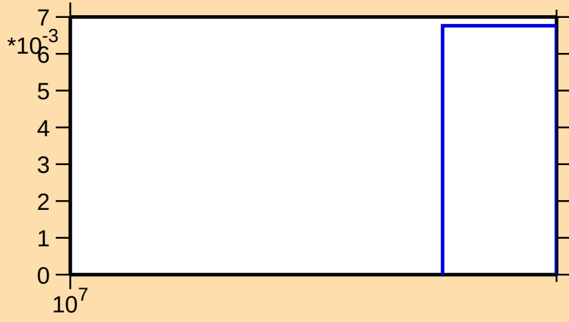
\sigma vs. E for ^{177}\text{Re}(n,3n)
