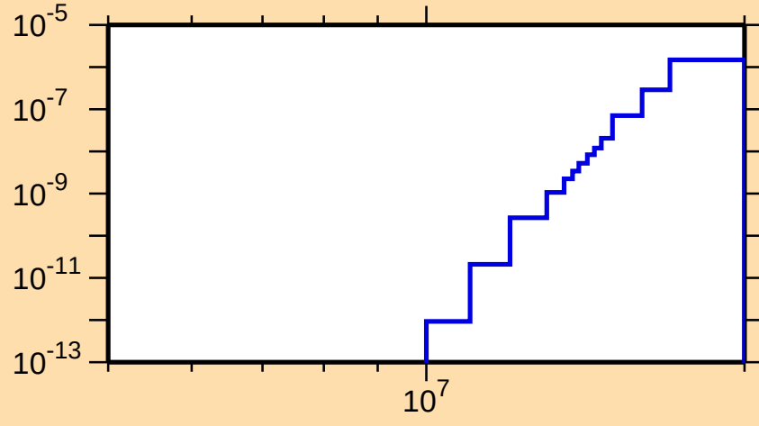
\sigma vs. E for ^{177}\text{Re}(n,\text{He3})
