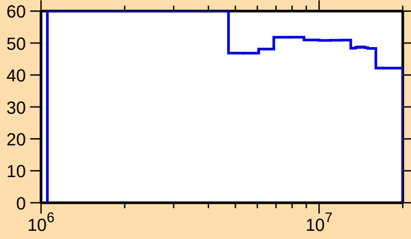
\Delta\sigma/\sigma vs. E for ^{177}\text{Re}(n,n_1)
