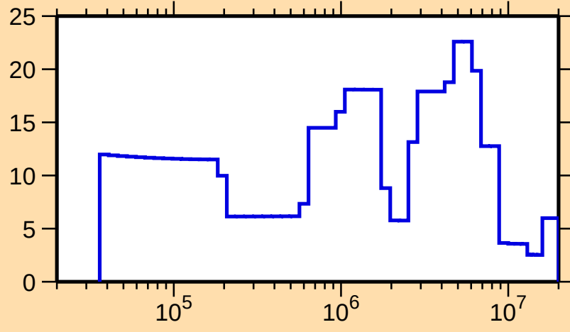
\Delta\sigma/\sigma vs. E for ^{177}\text{Re}(n,\text{el.})
