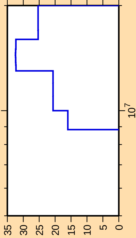
\Delta\sigma/\sigma vs. E for ^{177}\text{Re}(n,n\text{cont.})
