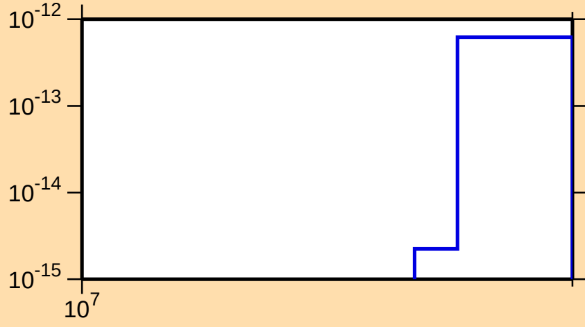
\sigma vs. E for ^{177}\text{Re}(\text{mt } 34)
