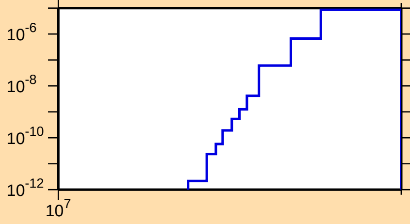
\sigma vs. E for ^{177}\text{Re}(n,\text{nd})
