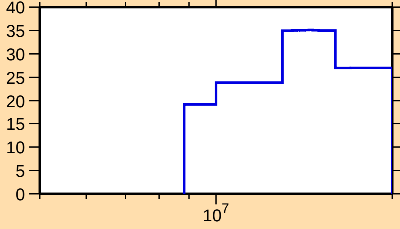
\Delta\sigma/\sigma vs. E for ^{177}\text{Re}(n,\text{inel.})
