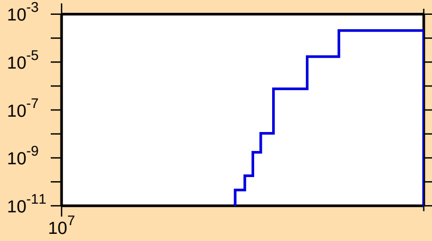
\sigma vs. E for ^{177}\text{Re}(n,2np)
