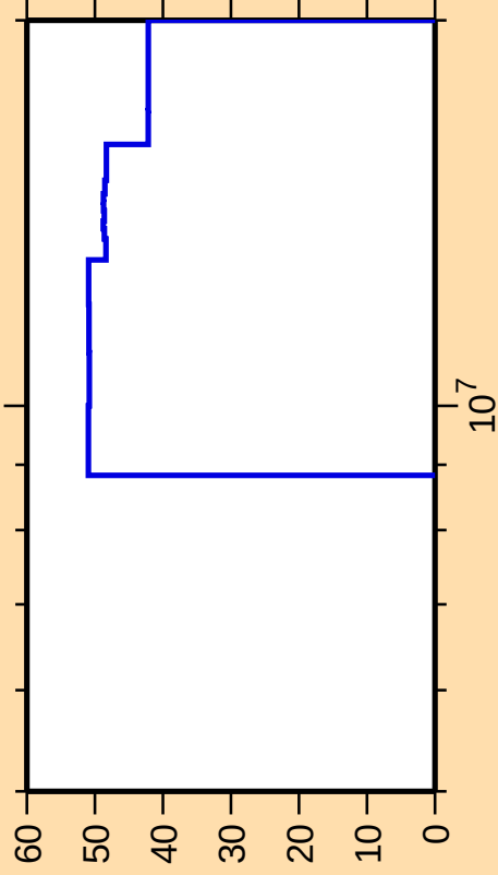
\Delta\sigma/\sigma vs. E for ^{177}\text{Re}(n,n_1)
