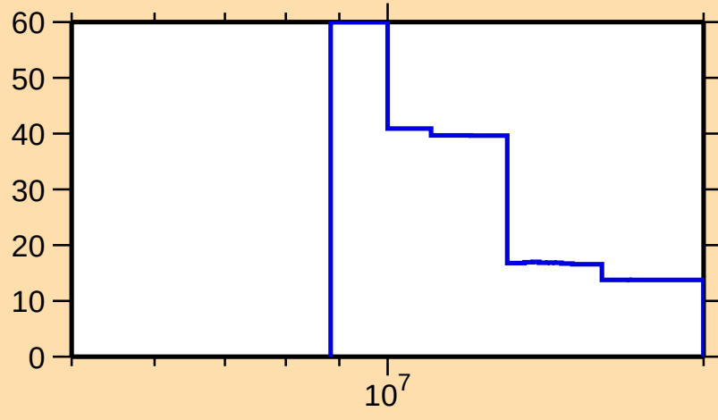
\Delta\sigma/\sigma vs. E for ^{177}\text{Re}(n,2n)
