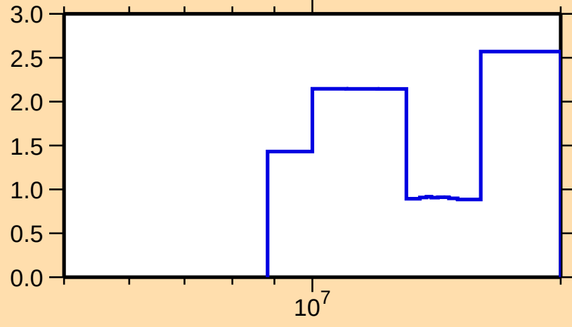
\Delta\sigma/\sigma vs. E for ^{177}\text{Re}(n,\text{tot.})
