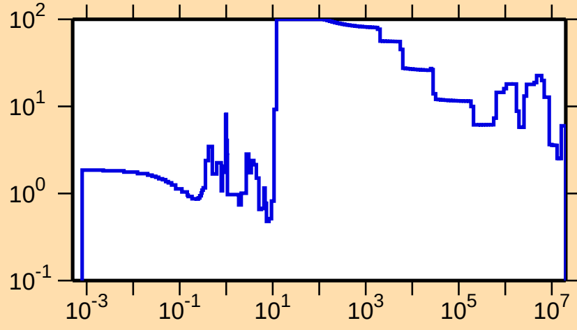
\Delta\sigma/\sigma vs. E for ^{177}\text{Re}(n,\text{el.})
