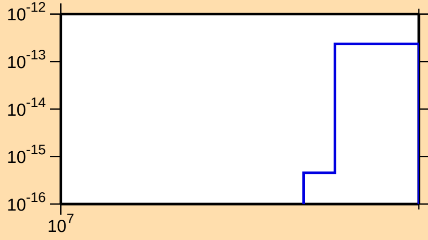
\sigma vs. E for ^{177}\text{Re}(n,\text{pt})
