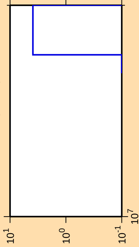
\Delta\sigma/\sigma vs. E for ^{177}\text{Re}(\text{mt } 34)
