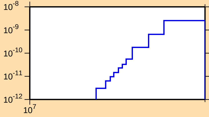
\sigma vs. E for ^{177}\text{Re}(\text{mt117})
