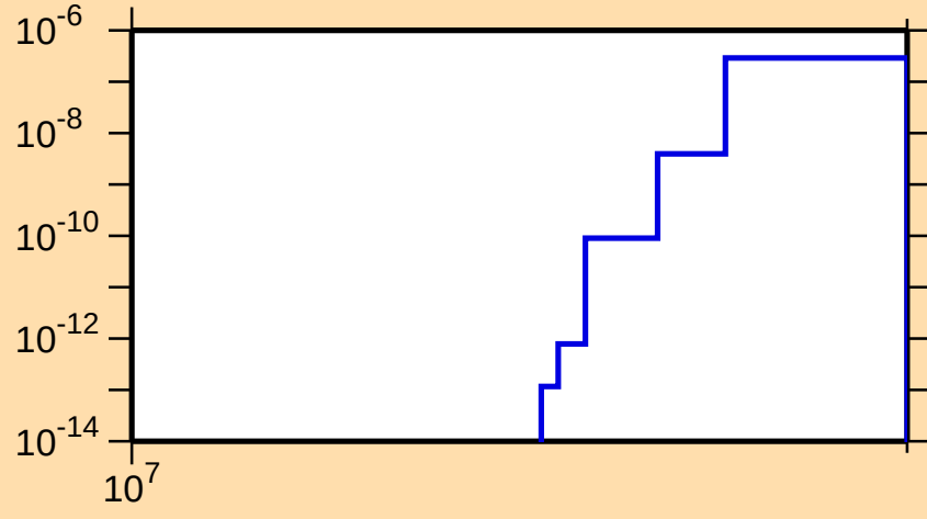
\sigma vs. E for ^{177}\text{Re}(n,nt)
