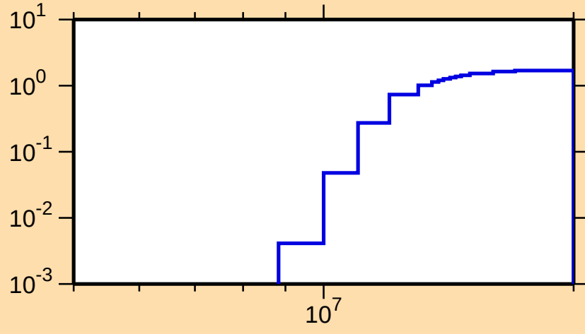
\sigma vs. E for ^{177}\text{Re}(n,2n)
