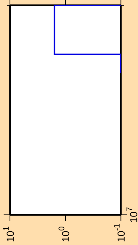
\Delta\sigma/\sigma vs. E for ^{177}\text{Re}(n,\text{pt})
