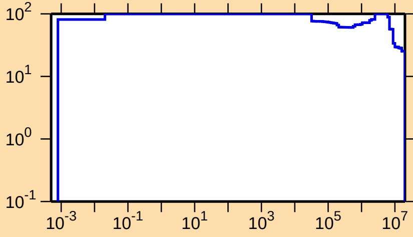
\Delta\sigma/\sigma vs. E for ^{177}\text{Re}(n,p)
