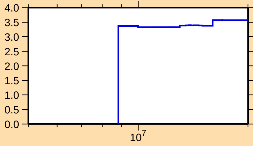
\Delta\sigma/\sigma vs. E for ^{177}\text{Re}(n,\text{nonel.})
