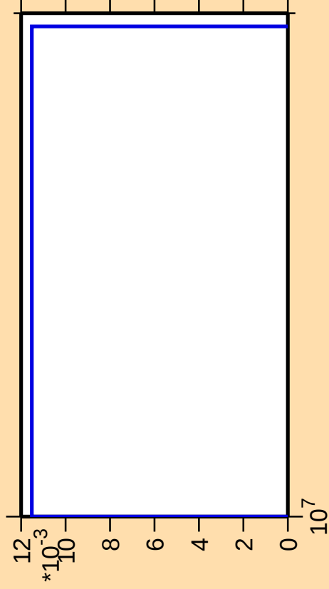
\Delta\sigma/\sigma vs. E for ^{177}\text{Re}(n,\text{pt})
