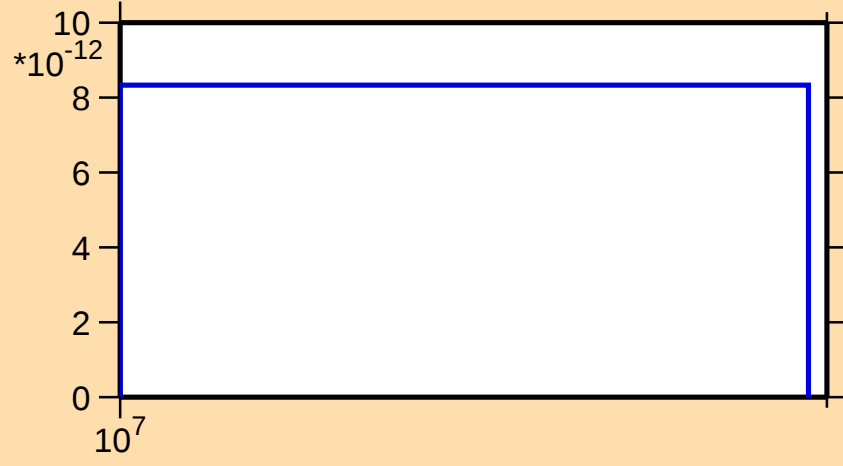
\sigma vs. E for ^{177}\text{Re}(n,\text{pd})
