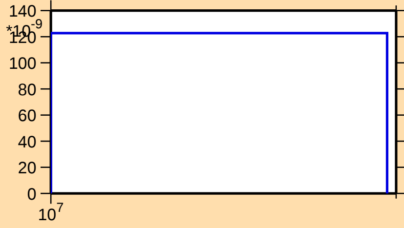
\sigma vs. E for ^{177}\text{Re}(n,\text{nd})
