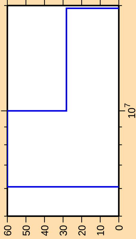
\Delta\sigma/\sigma vs. E for ^{177}\text{Re}(n,p)
