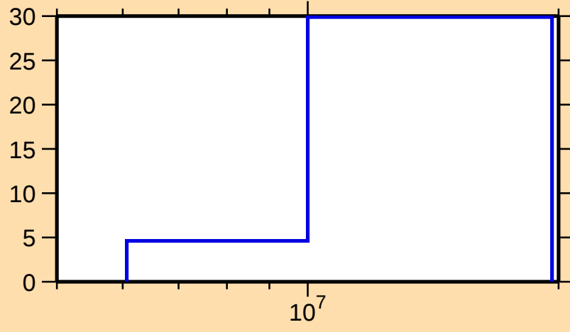
\Delta\sigma/\sigma vs. E for ^{177}\text{Re}(n,\text{inel.})
