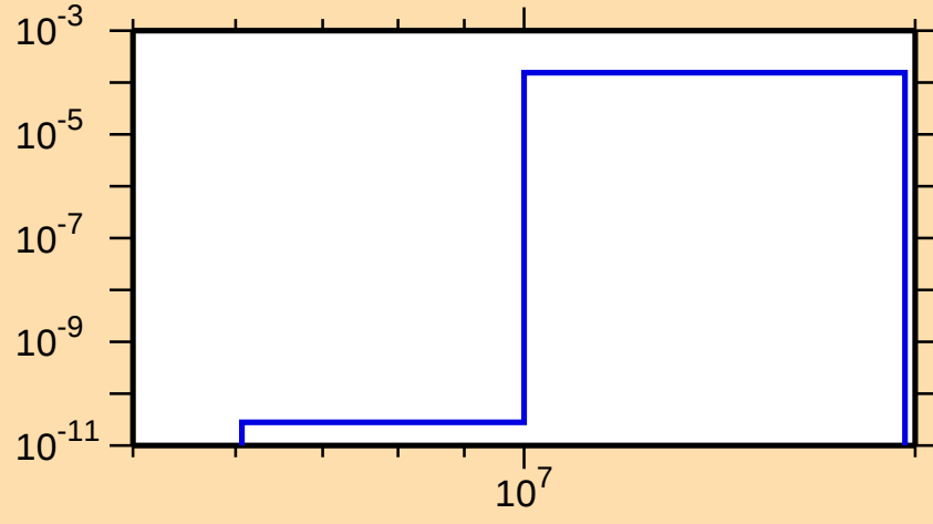
\sigma vs. E for ^{177}\text{Re}(n,t)
