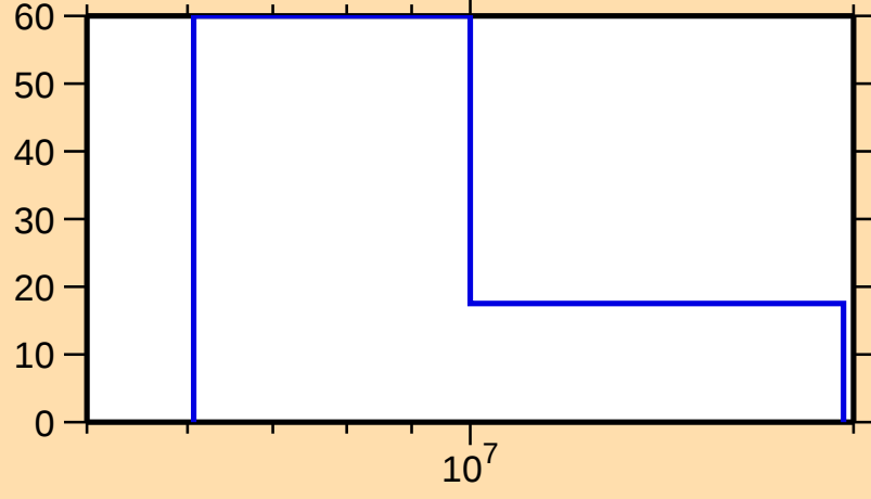
\Delta\sigma/\sigma vs. E for ^{177}\text{Re}(n,2n)
