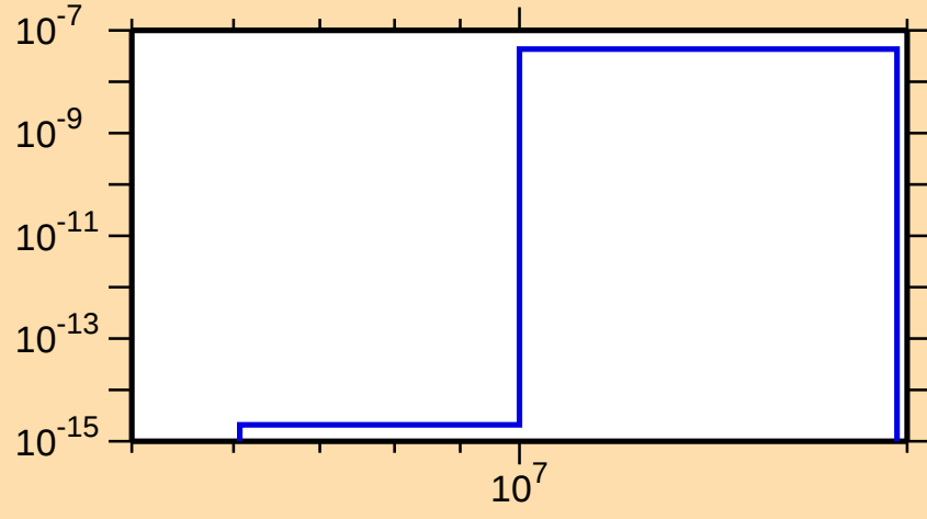
\sigma vs. E for ^{177}\text{Re}(n,\text{He3})
