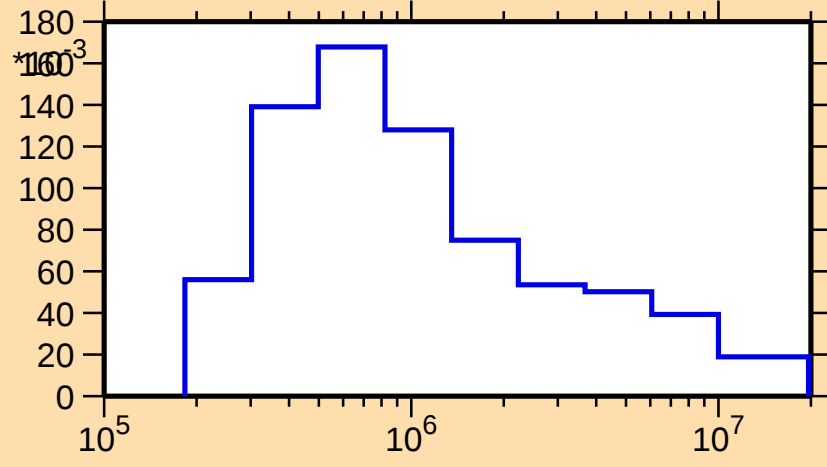
\sigma vs. E for ^{177}\text{Re}(n,n_4)
