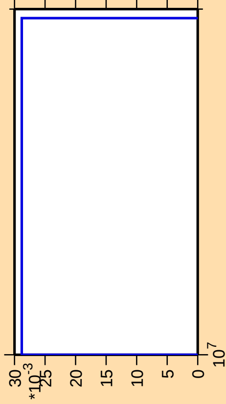
\Delta\sigma/\sigma vs. E for ^{177}\text{Re}(\text{mt } 34)
