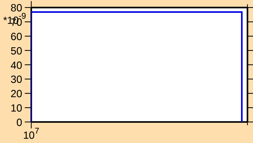
\sigma vs. E for ^{177}\text{Re}(n,2n\alpha)
