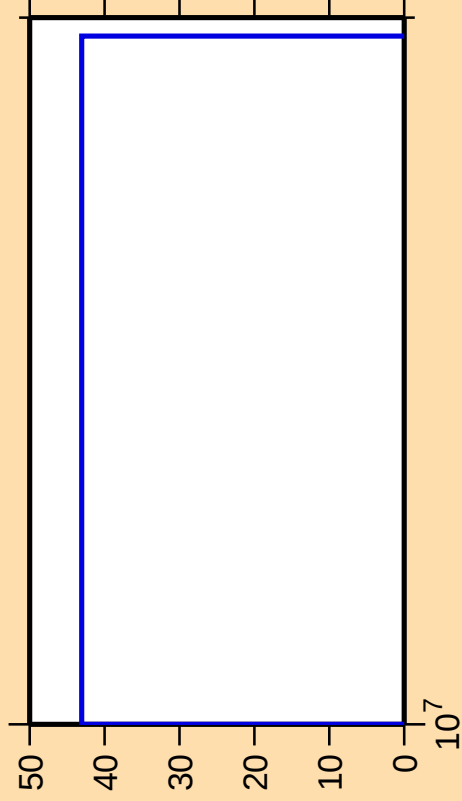
\Delta\sigma/\sigma vs. E for ^{177}\text{Re}(n,\text{pd})
