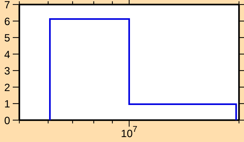
\Delta\sigma/\sigma vs. E for ^{177}\text{Re}(n,\text{tot.})
