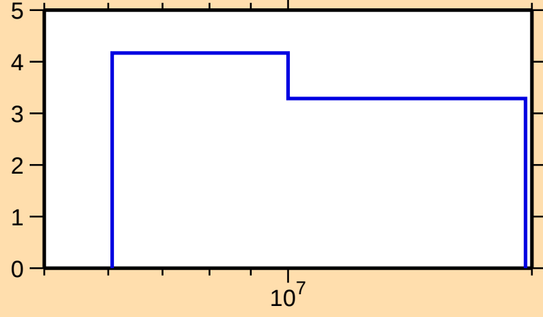
\Delta\sigma/\sigma vs. E for ^{177}\text{Re}(n,\text{nonel.})
