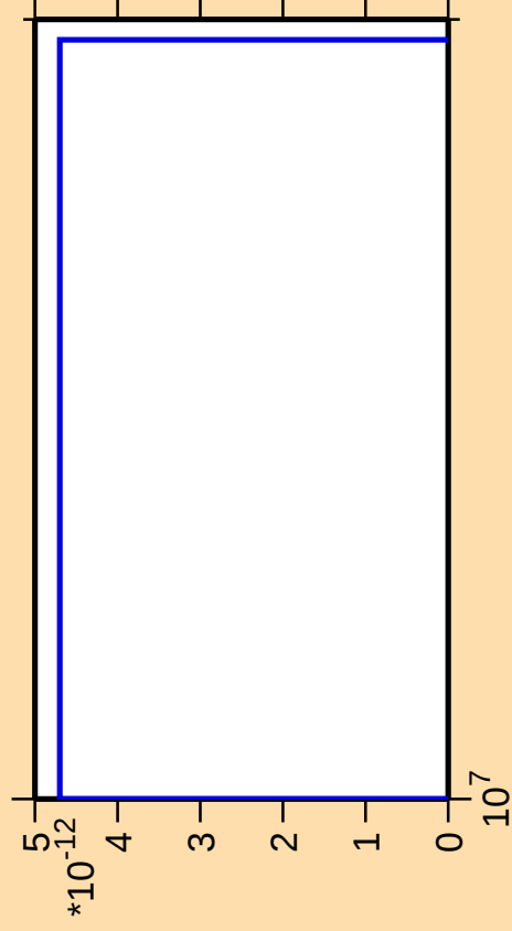
\Delta\sigma/\sigma vs. E for ^{177}\text{Re}(\text{mt } 42)
