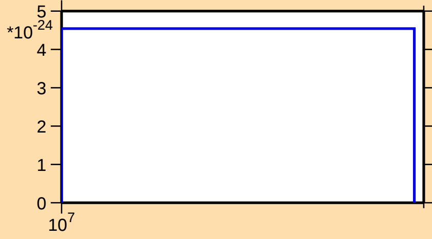
\sigma vs. E for ^{177}\text{Re}(\text{mt } 42)
