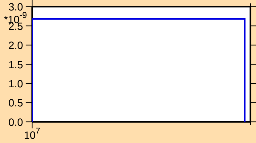
\sigma vs. E for ^{177}\text{Re}(n,nt)
