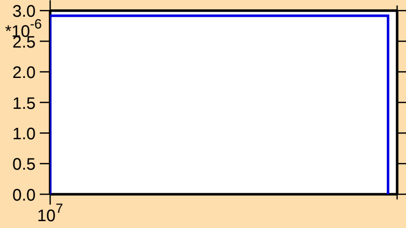
\sigma vs. E for ^{177}\text{Re}(n,2np)
