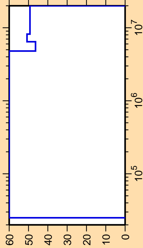
\Delta\sigma/\sigma vs. E for ^{177}\text{Re}(n,n_2)
