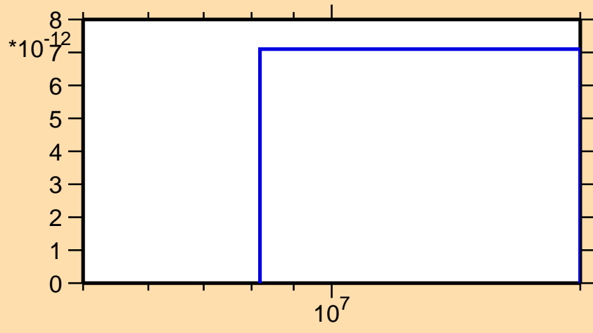
\sigma vs. E for ^{177}\text{Re}(n,pd)
