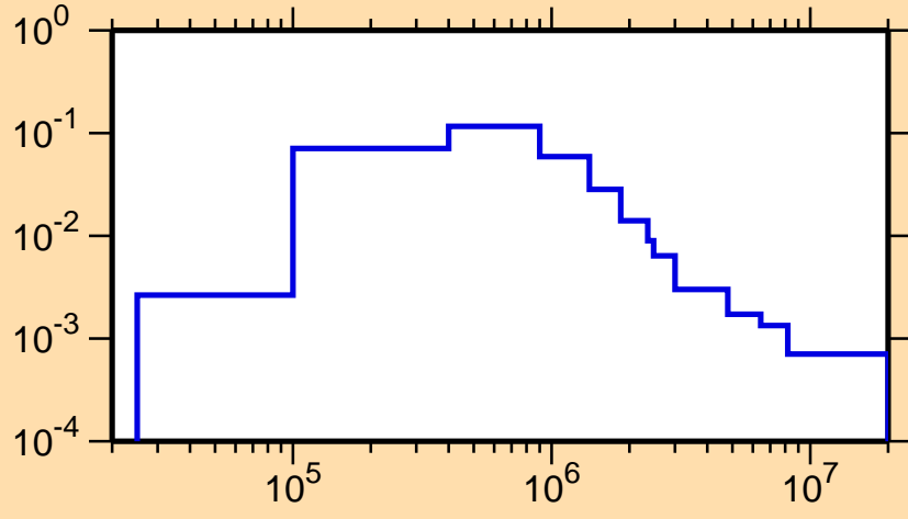
\sigma vs. E for ^{177}\text{Re}(n,n_2)
