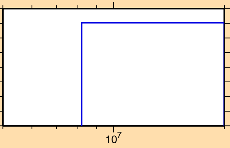
\sigma vs. E for ^{177}\text{Re}(n,\text{He3})
