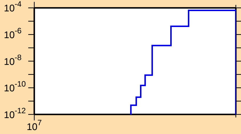
\sigma vs. E for ^{179}\text{Re}(n,2np)
