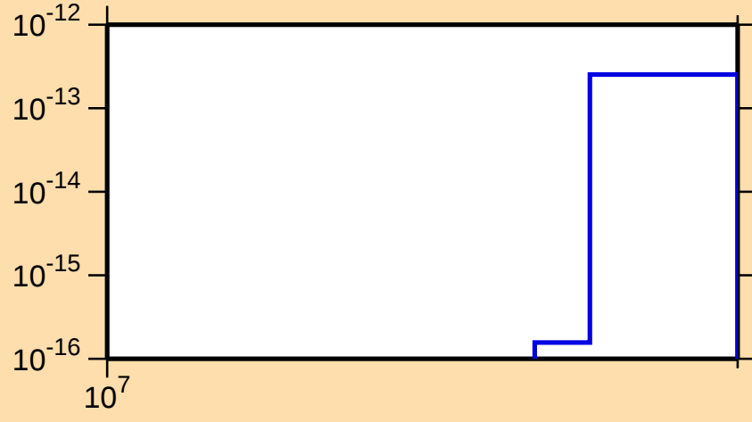
\sigma vs. E for ^{179}\text{Re}(\text{mt 34})
