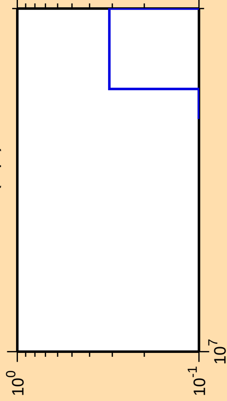
\Delta\sigma/\sigma vs. E for ^{179}\text{Re}(n,\text{pt})
