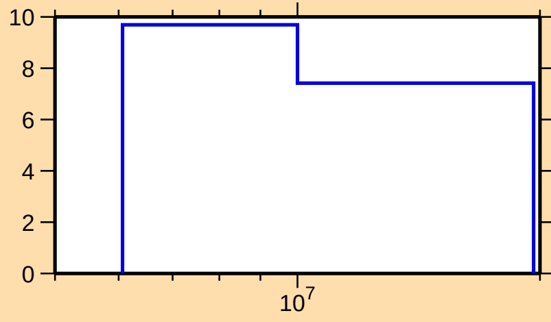
\Delta\sigma/\sigma vs. E for ^{179}\text{Re}(n,\text{nonel.})
