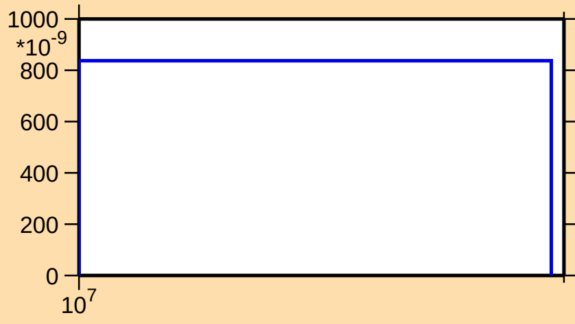
\sigma vs. E for ^{179}\text{Re}(n,2np)
