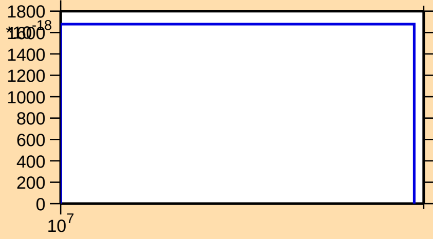
\sigma vs. E for ^{179}\text{Re}(\text{mt } 34)
