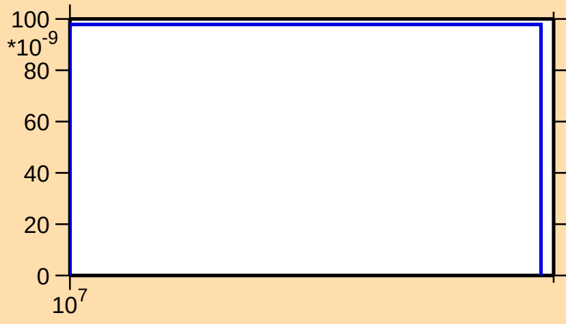
\sigma vs. E for ^{179}\text{Re}(n,\text{nd})
