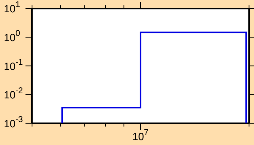
\sigma vs. E for ^{179}\text{Re}(n,2n)
