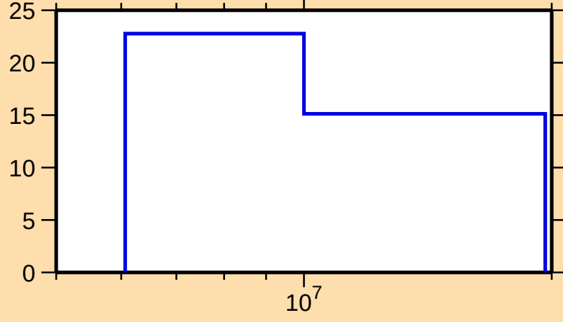
\Delta\sigma/\sigma vs. E for ^{179}\text{Re}(n,\text{el.})
