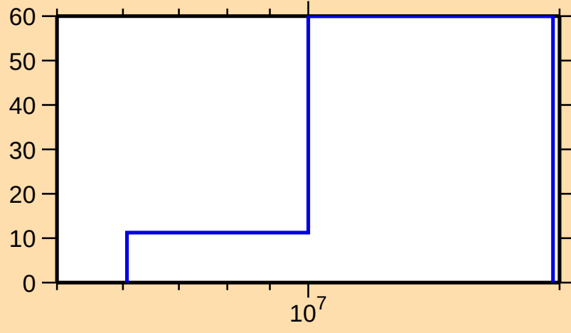
\Delta\sigma/\sigma vs. E for ^{179}\text{Re}(n,\text{inel.})
