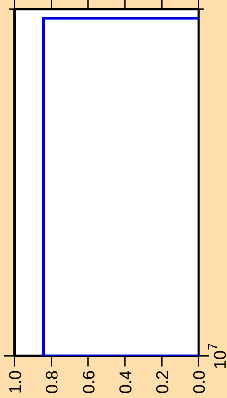
\Delta\sigma/\sigma vs. E for ^{179}\text{Re}(n,\text{pd})
