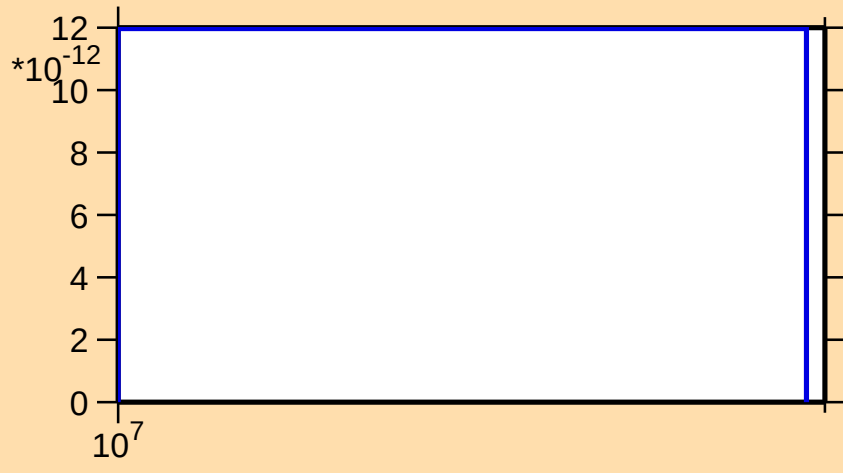
\sigma vs. E for ^{179}\text{Re}(\text{mt117})
