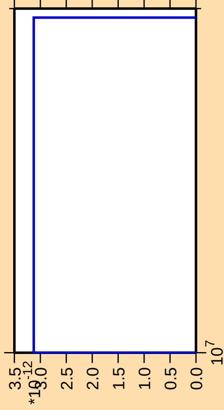
\Delta\sigma/\sigma vs. E for ^{179}\text{Re}(\text{mt } 42)
