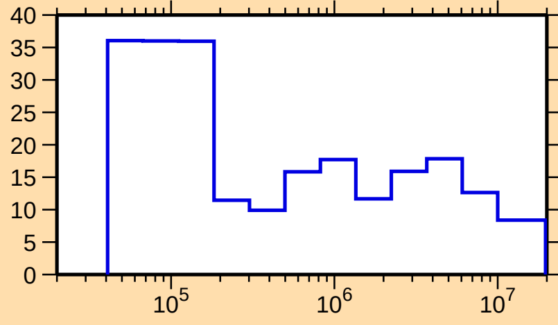
\Delta\sigma/\sigma vs. E for ^{179}\text{Re}(n,\text{tot.})
