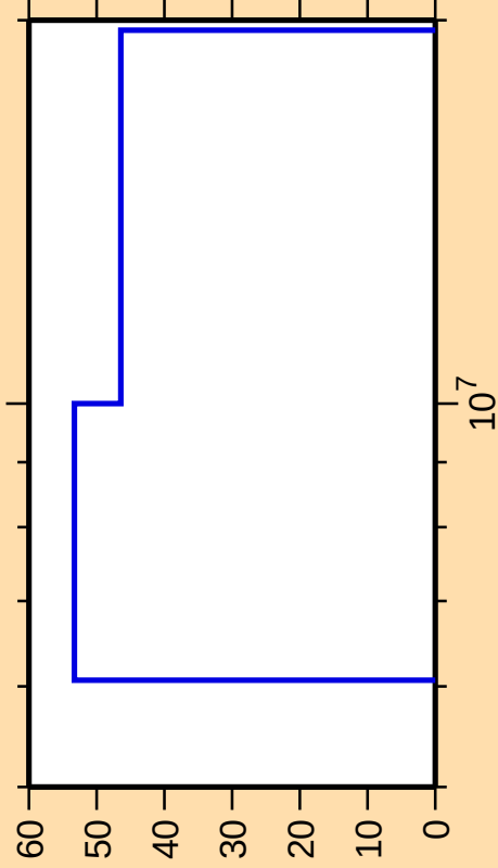
\Delta\sigma/\sigma vs. E for ^{179}\text{Re}(n,p)
