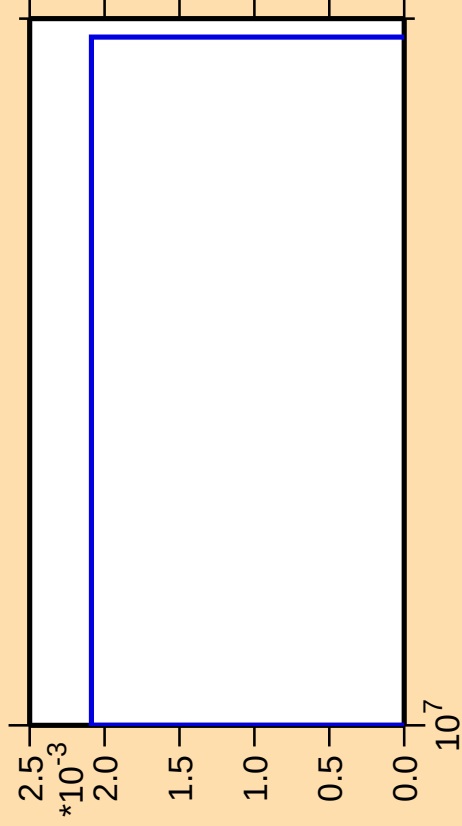
\Delta\sigma/\sigma vs. E for ^{179}\text{Re}(n,\text{pt})
