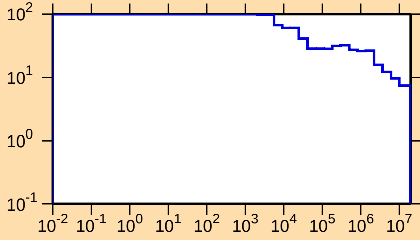
\Delta\sigma/\sigma vs. E for ^{179}\text{Re}(n,\text{nonel.})
