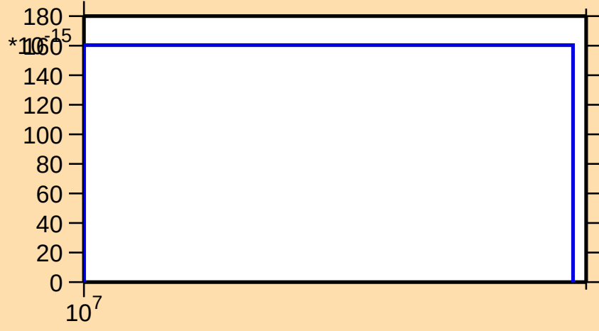
\sigma vs. E for ^{179}\text{Re}(n,\text{pd})
