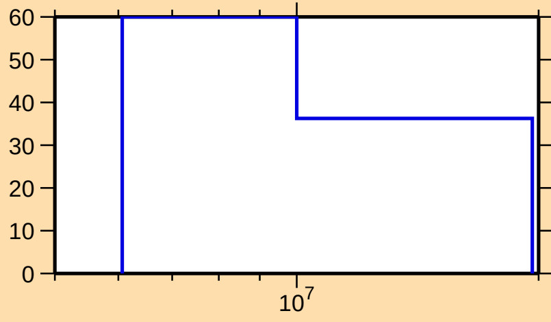
\Delta\sigma/\sigma vs. E for ^{179}\text{Re}(n,2n)
