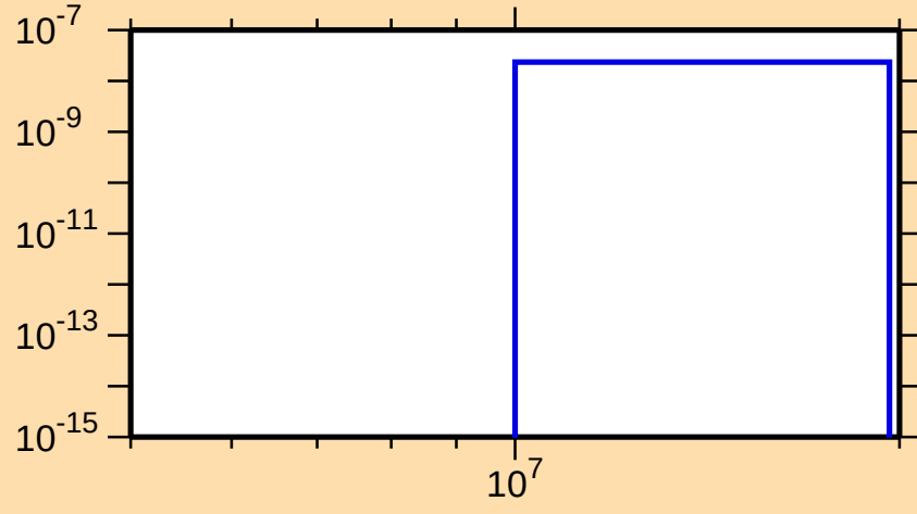
\sigma vs. E for ^{179}\text{Re}(n,2n\alpha)
