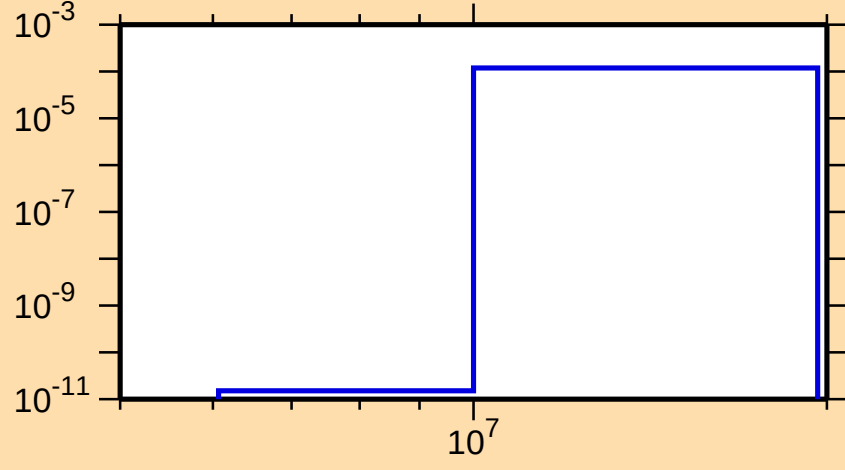
\sigma vs. E for ^{179}\text{Re}(n,t)
