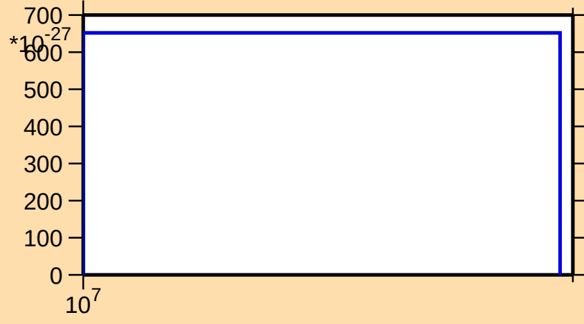
\sigma vs. E for ^{179}\text{Re}(\text{mt } 42)
