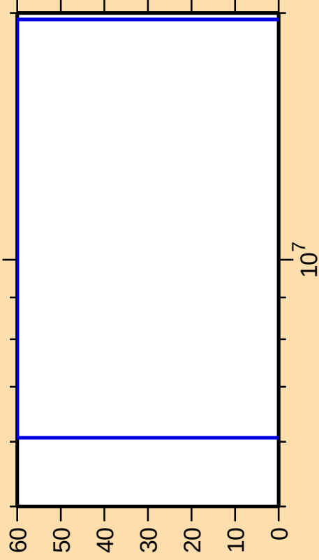
\Delta\sigma/\sigma vs. E for ^{179}\text{Re}(n,t)
