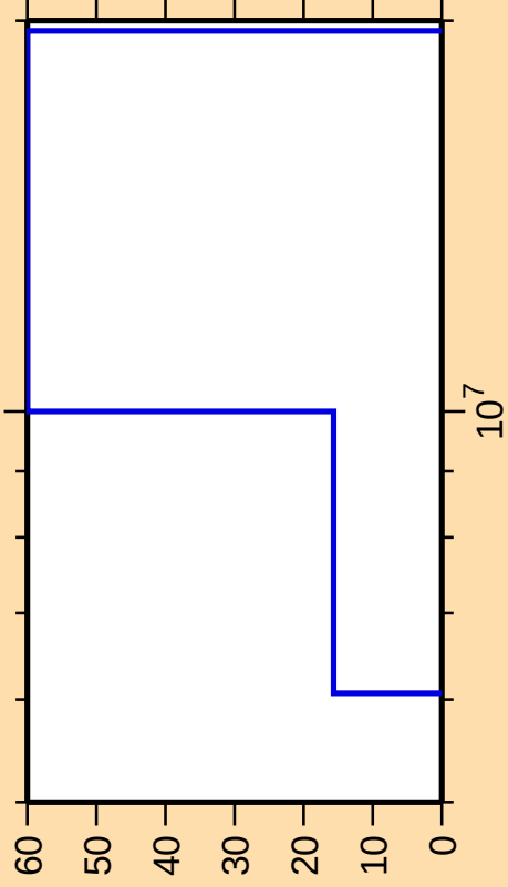
\Delta\sigma/\sigma vs. E for ^{179}\text{Re}(n,n\text{cont.})
