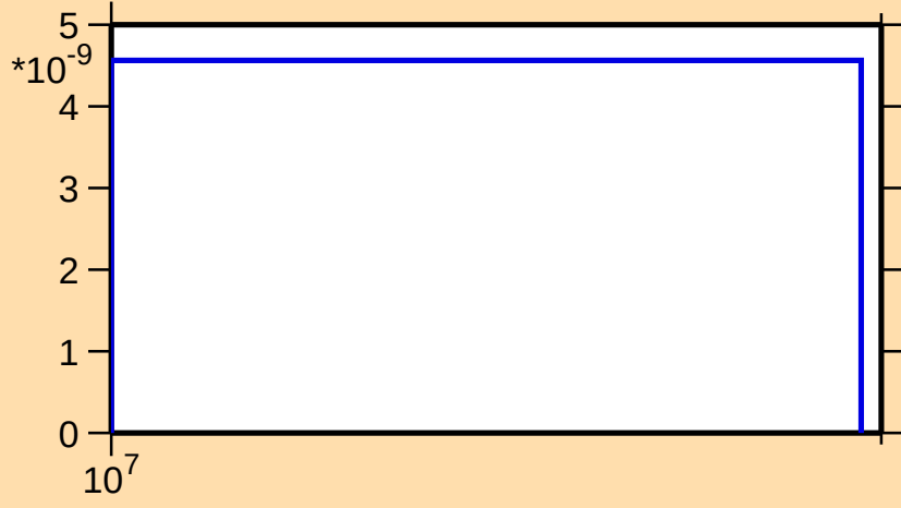
\sigma vs. E for ^{179}\text{Re}(n,nt)
