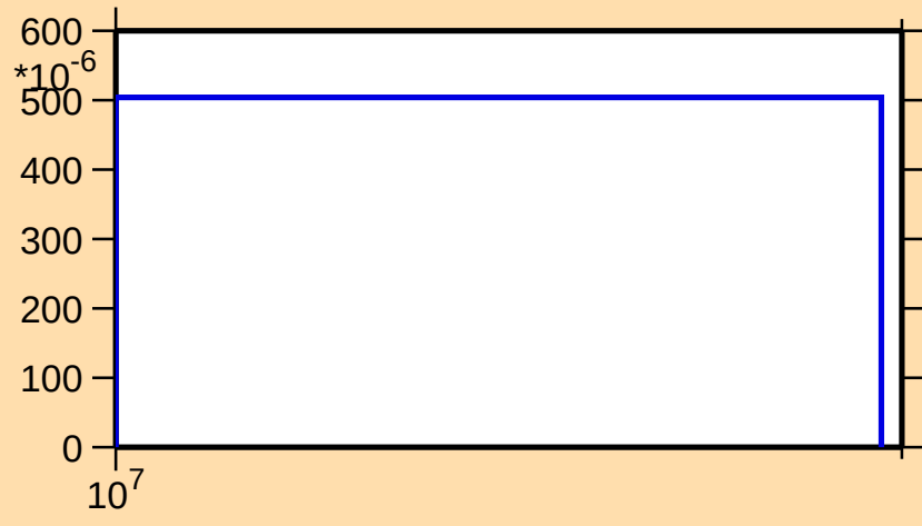
\sigma vs. E for ^{179}\text{Re}(n,3n)
