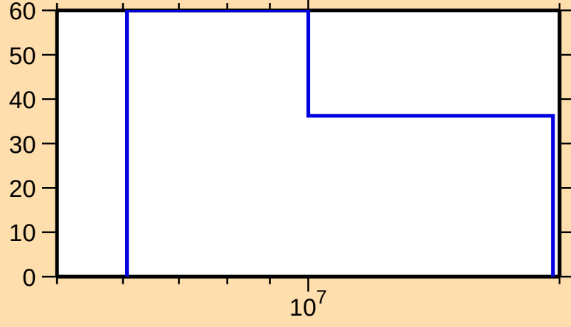
\Delta\sigma/\sigma vs. E for ^{179}\text{Re}(n,2n)
