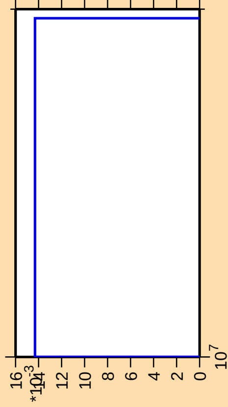
\Delta\sigma/\sigma vs. E for ^{179}\text{Re}(\text{mt } 34)
