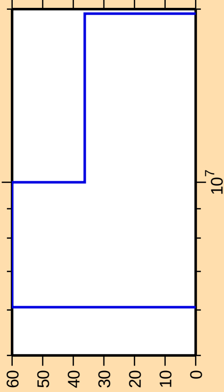
\Delta\sigma/\sigma vs. E for ^{179}\text{Re}(n,2n)
