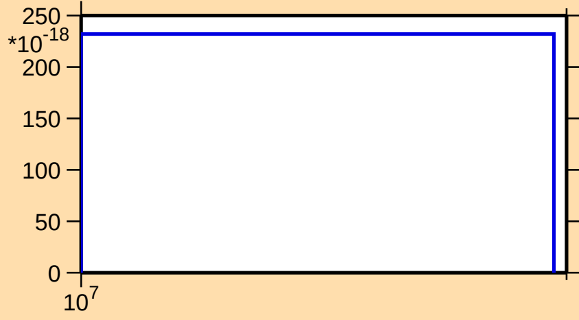
\sigma vs. E for ^{179}\text{Re}(n,\text{pt})
