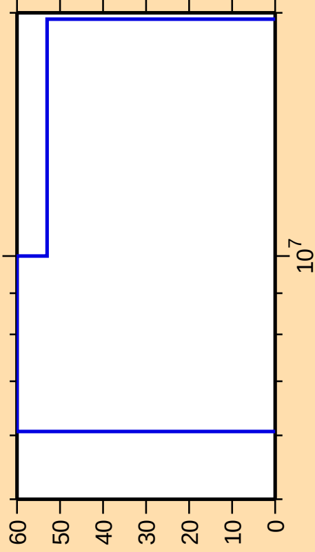
\Delta\sigma/\sigma vs. E for ^{179}\text{Re}(n,n_1)
