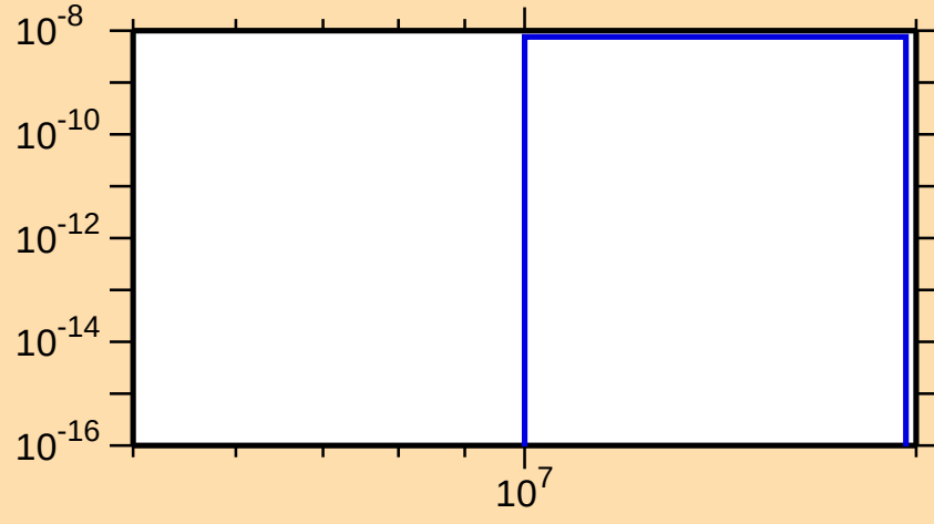
\sigma vs. E for ^{179}\text{Re}(n,\text{He3})
