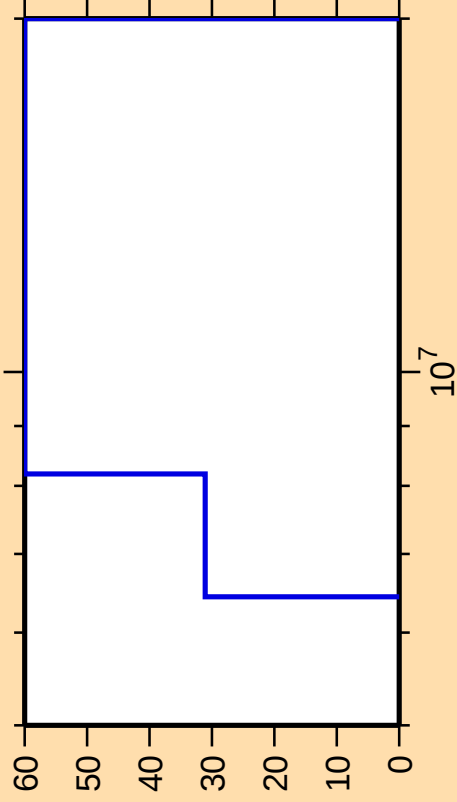
\Delta\sigma/\sigma vs. E for ^{179}\text{Re}(n,p\alpha)
