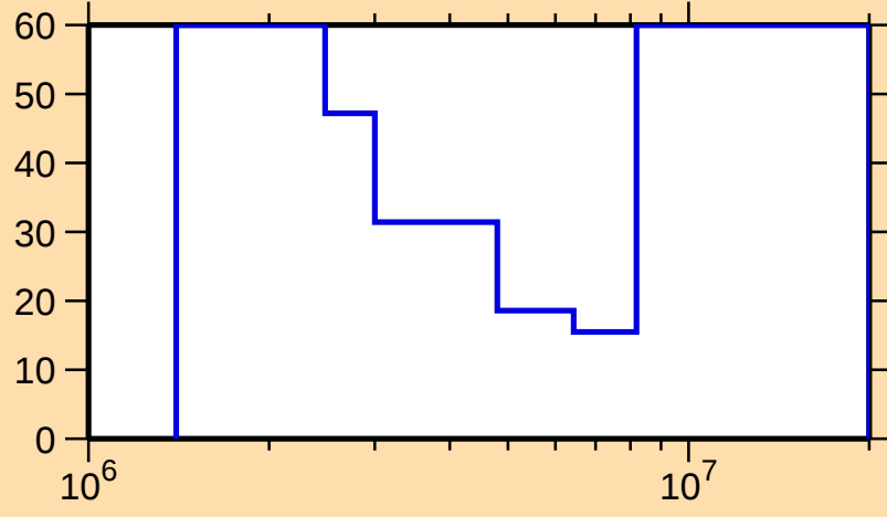
\Delta\sigma/\sigma vs. E for ^{179}\text{Re}(n,n\text{cont.})
