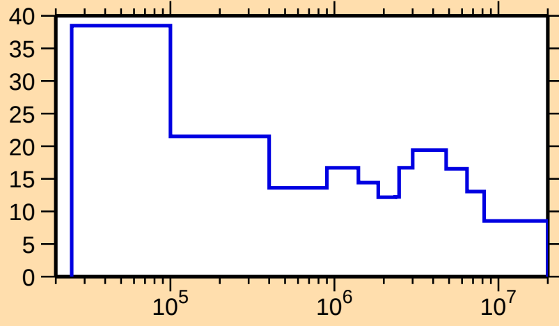
\Delta\sigma/\sigma vs. E for ^{179}\text{Re}(n,\text{tot.})
