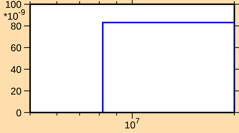
\sigma vs. E for ^{179}\text{Re}(n,\text{nd})
