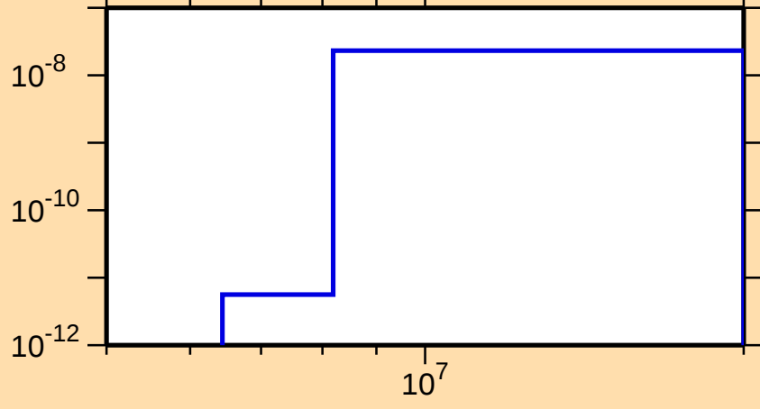
\sigma vs. E for ^{179}\text{Re}(n,p\alpha)
