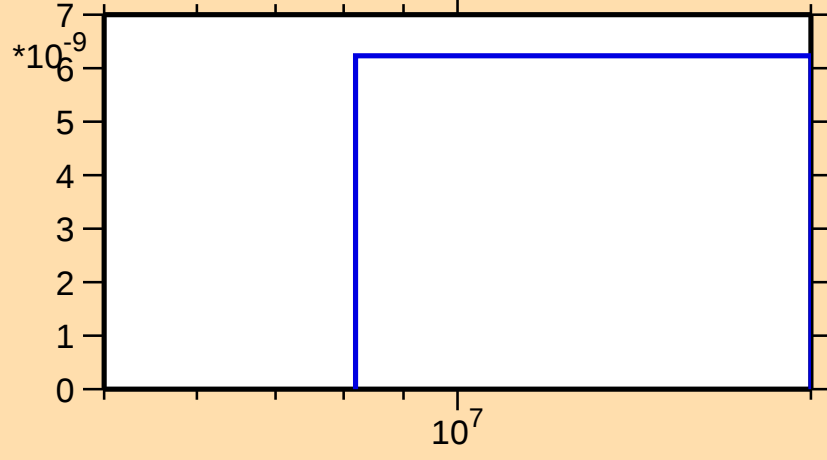
\sigma vs. E for ^{179}\text{Re}(n,\text{He3})
