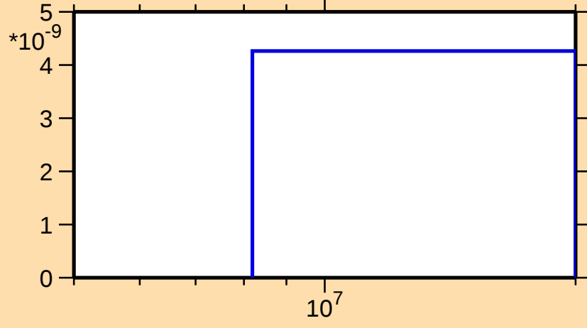
\sigma vs. E for ^{179}\text{Re}(n,nt)
