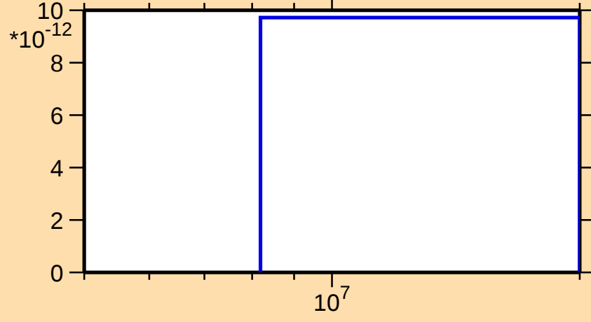
\sigma vs. E for ^{179}\text{Re}(\text{mt117})
