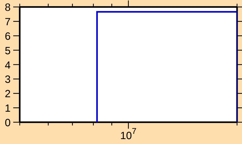
\Delta\sigma/\sigma vs. E for ^{179}\text{Re}(n,\text{nonel.})
