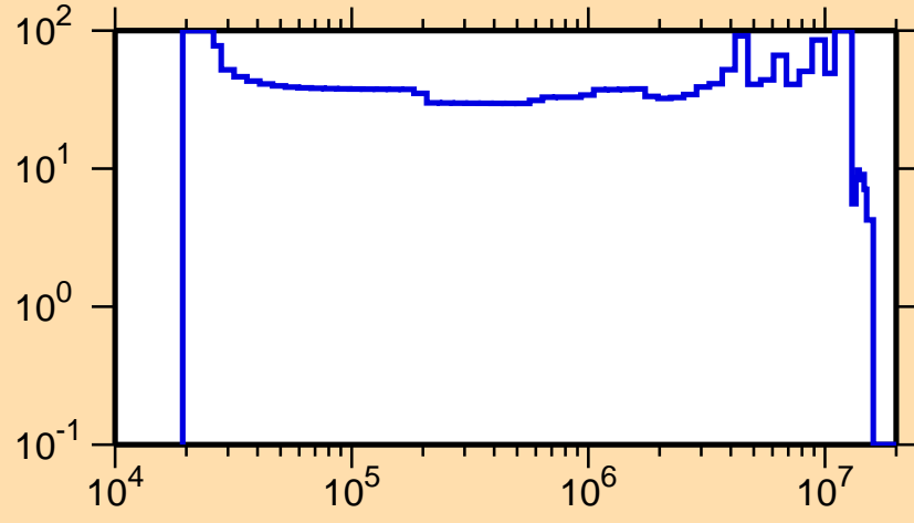
\Delta\sigma/\sigma vs. E for ^{180}\text{Re}(n,n_1)
