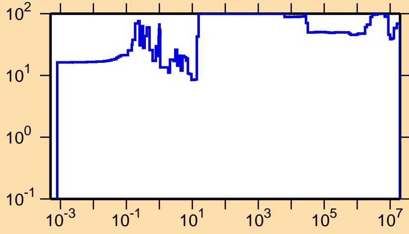
\Delta\sigma/\sigma vs. E for ^{180}\text{Re}(n,\gamma)
