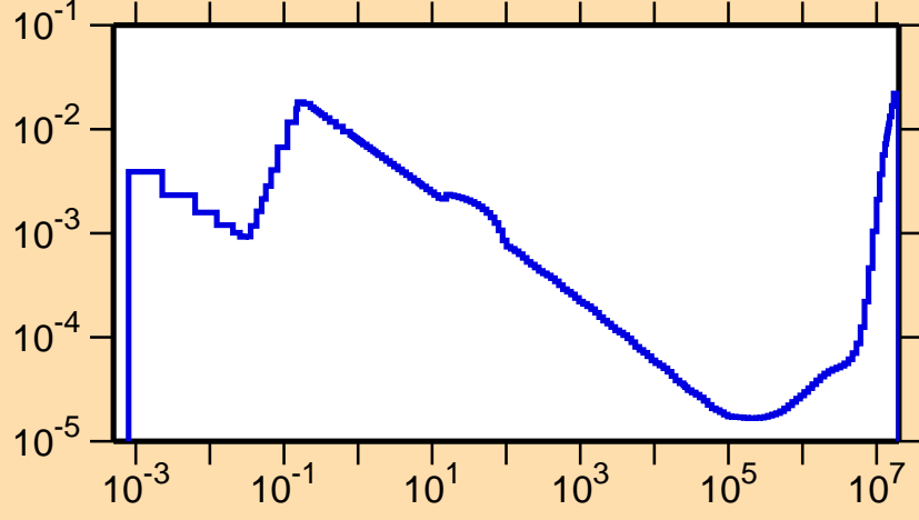
\sigma vs. E for ^{180}\text{Re}(n,\alpha)
