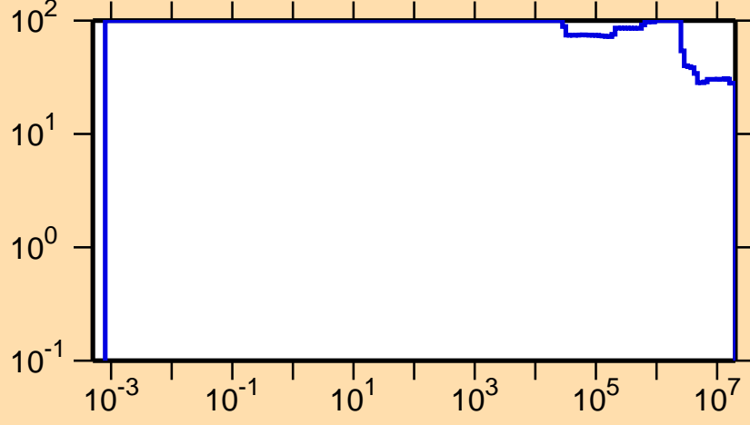
\Delta\sigma/\sigma vs. E for ^{180}\text{Re}(n,p)
