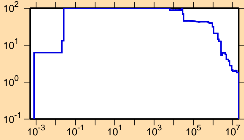
\Delta\sigma/\sigma vs. E for ^{180}\text{Re}(n,\text{nonel.})
