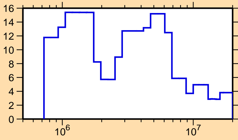
\Delta\sigma/\sigma vs. E for ^{180}\text{Re}(n, \text{el.})
