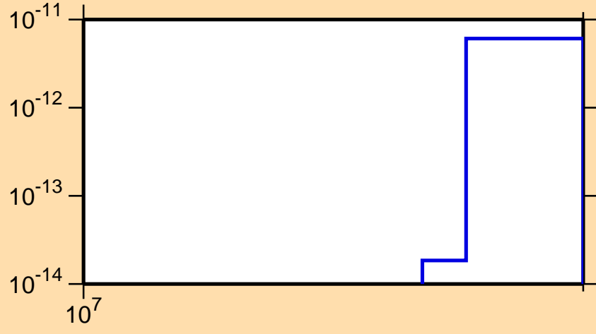
\sigma vs. E for ^{180}\text{Re}(\text{mt 34})
