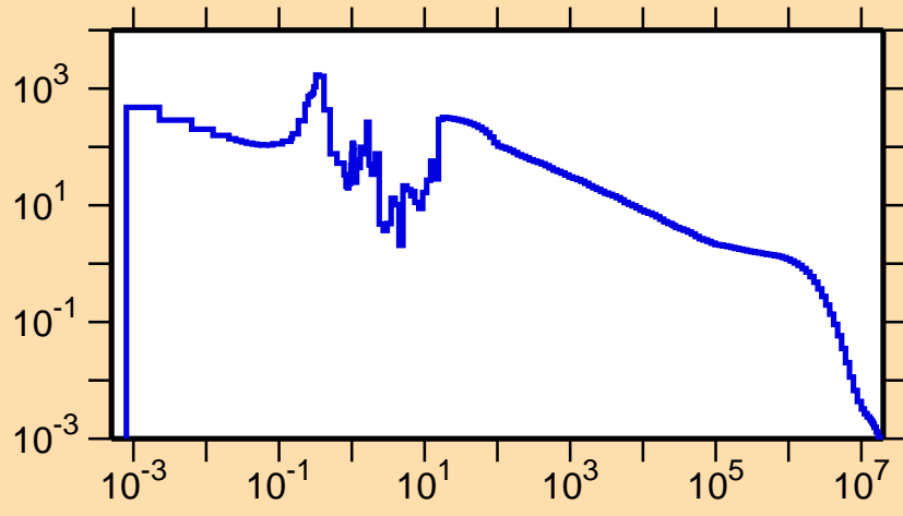
\sigma vs. E for ^{180}\text{Re}(n,\gamma)
