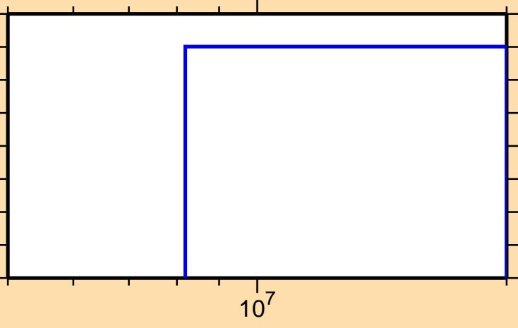
\sigma vs. E for ^{180}\text{Re}(n,2np)
