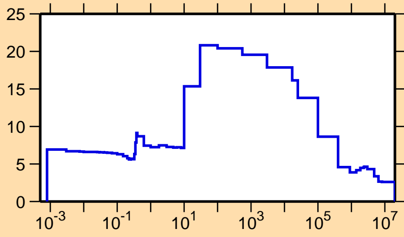
\sigma vs. E for ^{180}\text{Re}(n,\text{el.})
