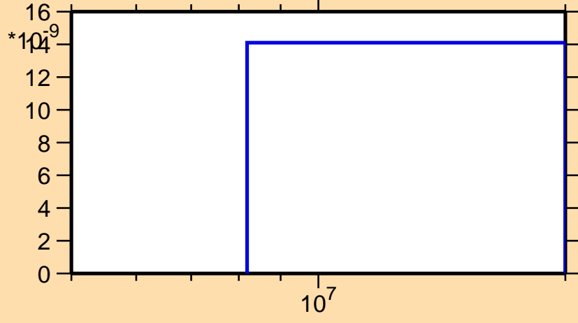
\sigma vs. E for ^{180}\text{Re}(n,\text{He3})
