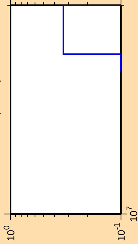
\Delta\sigma/\sigma vs. E for ^{184}\text{Re}(\text{mt 34})
