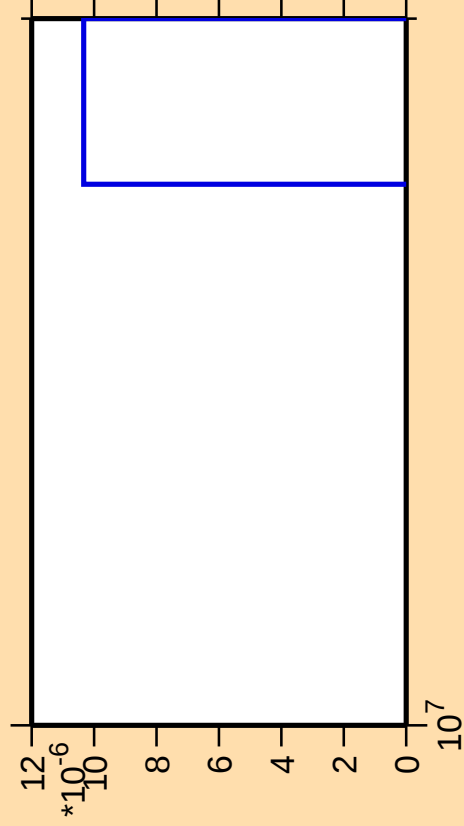
\Delta\sigma/\sigma vs. E for ^{184}\text{Re}(\text{mt } 42)
