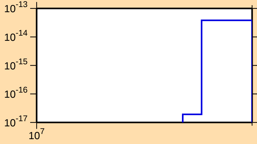
\sigma vs. E for ^{184}\text{Re}(\text{mt 34})
