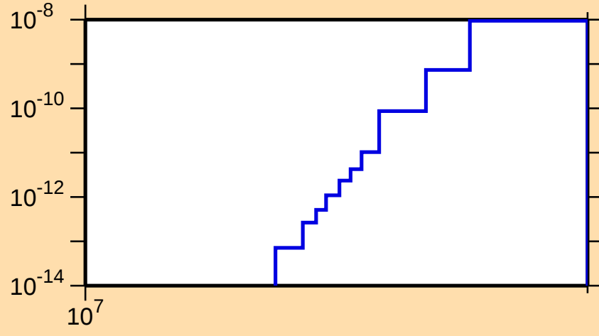
\sigma vs. E for ^{184}\text{Re}(n,\text{He3})
