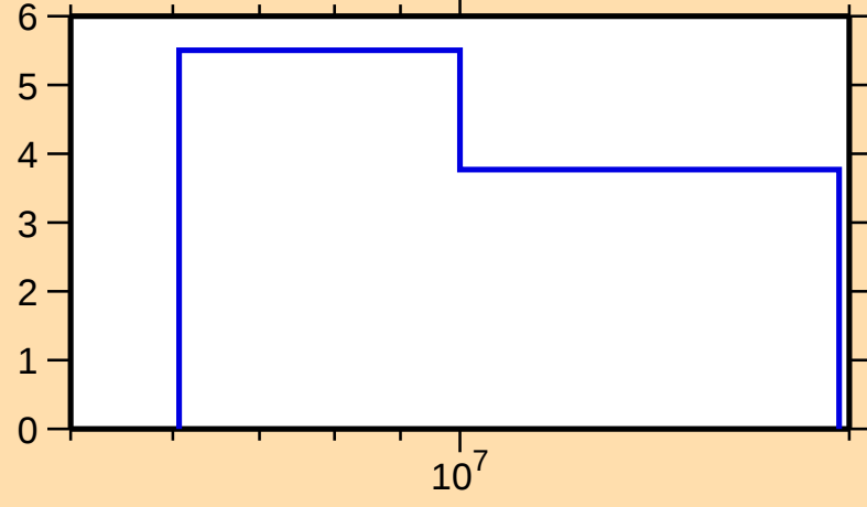
\Delta\sigma/\sigma vs. E for ^{184}\text{Re}(n,\text{tot.})
