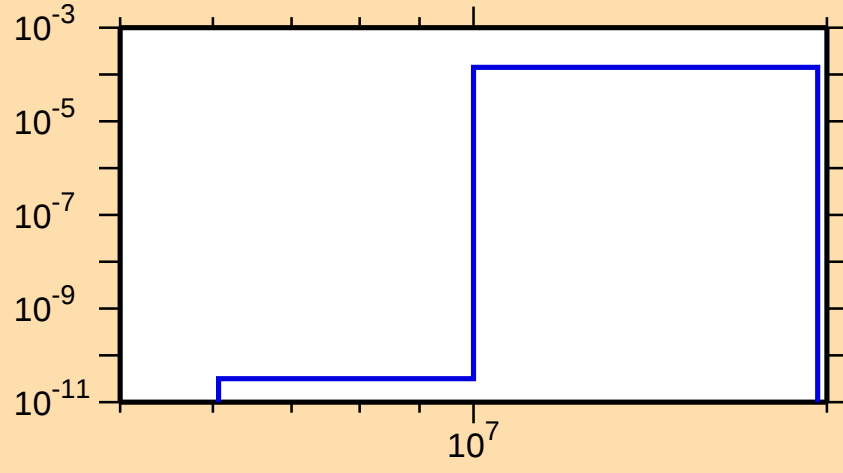
\sigma vs. E for ^{184}\text{Re}(n,t)
