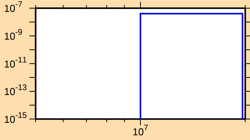
\sigma vs. E for ^{184}\text{Re}(n,2n\alpha)
