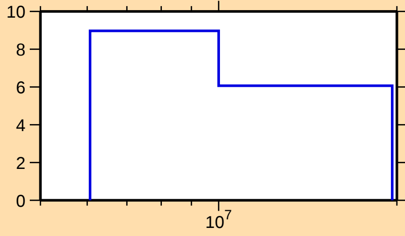
\Delta\sigma/\sigma vs. E for ^{184}\text{Re}(n,\text{nonel.})
