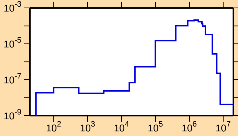
\sigma vs. E for ^{184}\text{Re}(n,n_3)
