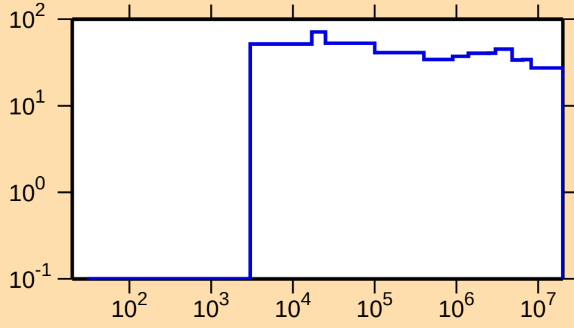
\Delta\sigma/\sigma vs. E for ^{184}\text{Re}(n,n_1)
