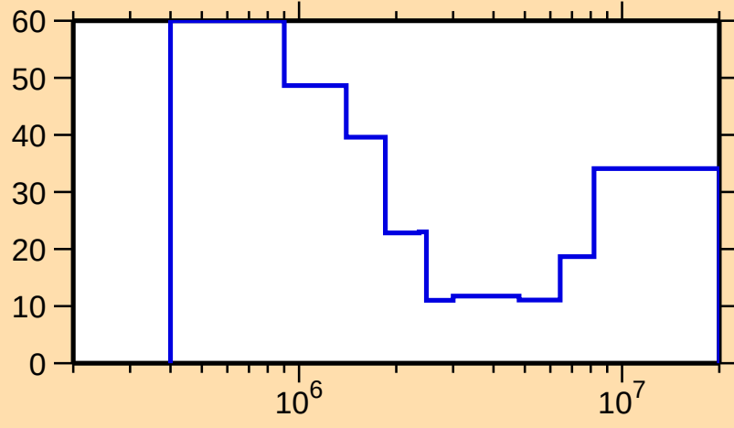
\Delta\sigma/\sigma vs. E for ^{184}\text{Re}(n,n\text{cont.})
