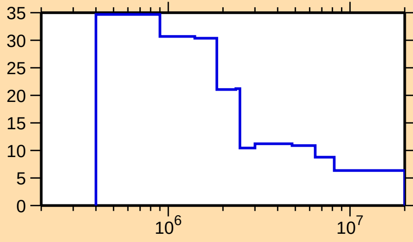
\Delta\sigma/\sigma vs. E for ^{184}\text{Re}(n,n\text{onel.})
