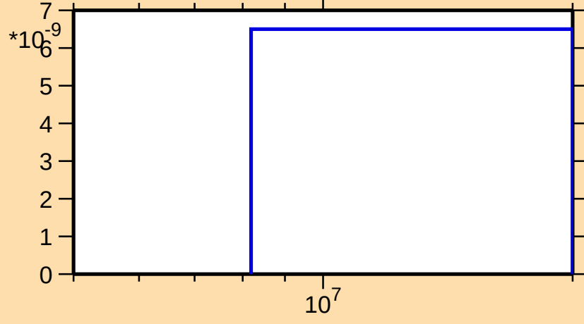
\sigma vs. E for ^{184}\text{Re}(n,nt)
