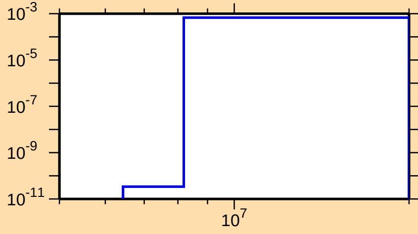
\sigma vs. E for ^{184}\text{Re}(n,np)
