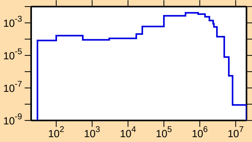
\sigma vs. E for ^{184}\text{Re}(n,n_4)
