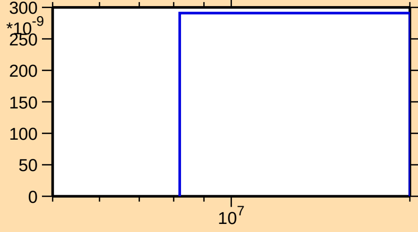
\sigma vs. E for ^{184}\text{Re}(n,\text{nd})
