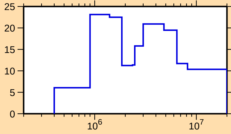
\Delta\sigma/\sigma vs. E for ^{184}\text{Re}(n,\text{el.})
