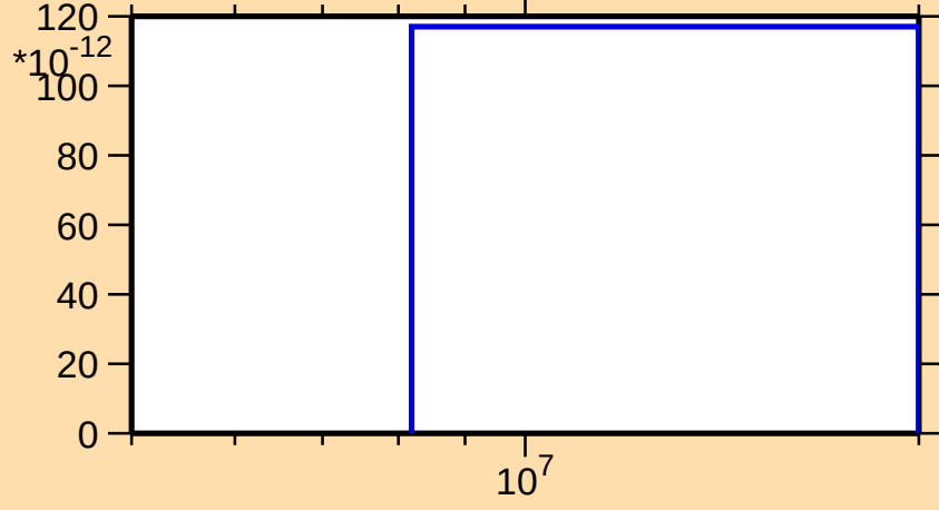
\sigma vs. E for ^{184}\text{Re}(n,\text{He3})
