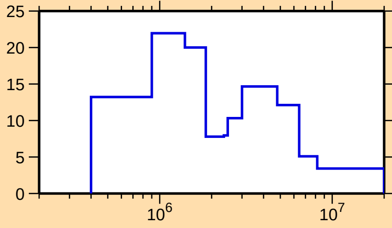
\Delta\sigma/\sigma vs. E for ^{184}\text{Re}(n,\text{tot.})
