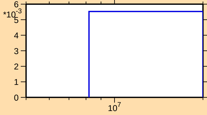
\sigma vs. E for ^{184}\text{Re}(n,3n)
