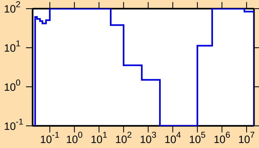
\Delta\sigma/\sigma vs. E for ^{184}\text{Re}(n,p)
