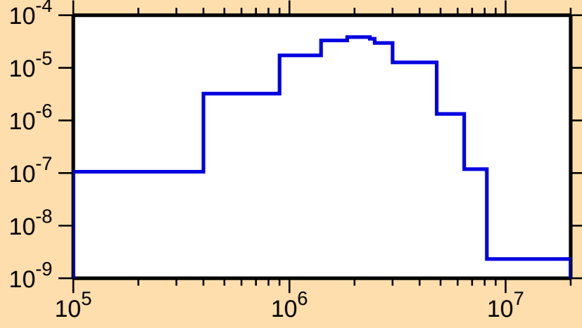
\sigma vs. E for ^{184}\text{Re}(n,n_2)
