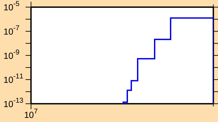
\sigma vs. E for ^{185}\text{Re}(n,nt)
