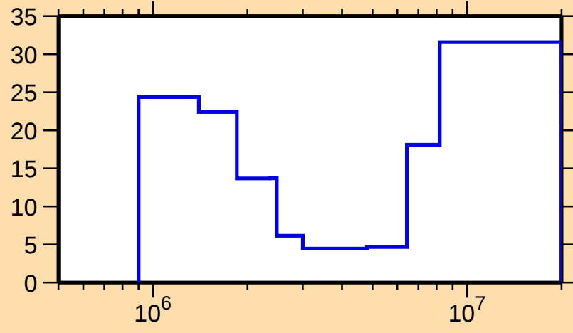
\Delta\sigma/\sigma vs. E for ^{185}\text{Re}(n,n\text{cont.})
