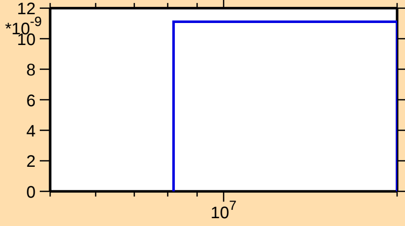
\sigma vs. E for ^{185}\text{Re}(n,nt)
