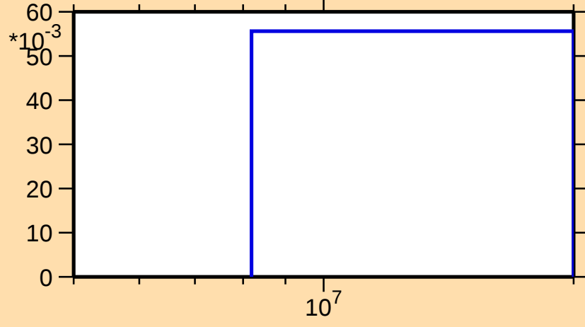
\sigma vs. E for ^{185}\text{Re}(n,3n)
