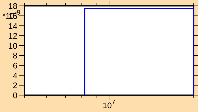
\sigma vs. E for ^{185}\text{Re}(n,\text{nd})
