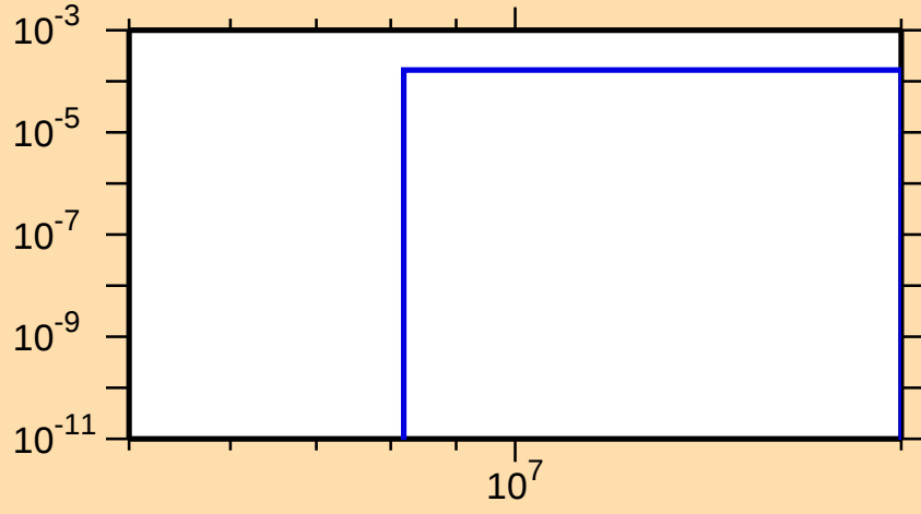
\sigma vs. E for ^{185}\text{Re}(n,t)
