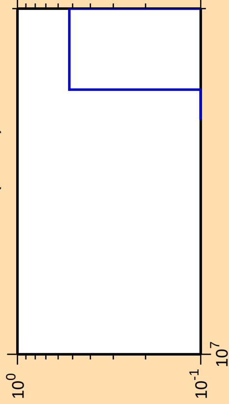
\Delta\sigma/\sigma vs. E for ^{188}\text{Re}(n,3n\alpha)
