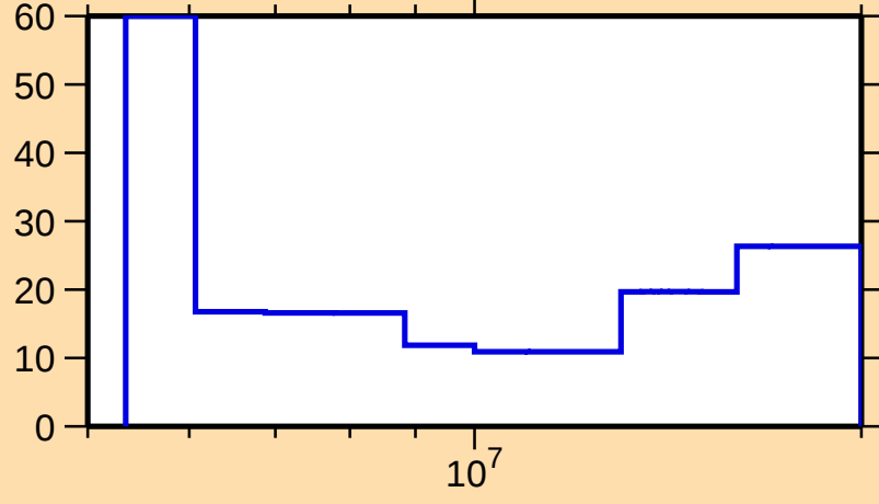
\Delta\sigma/\sigma vs. E for ^{188}\text{Re}(n,2n)
