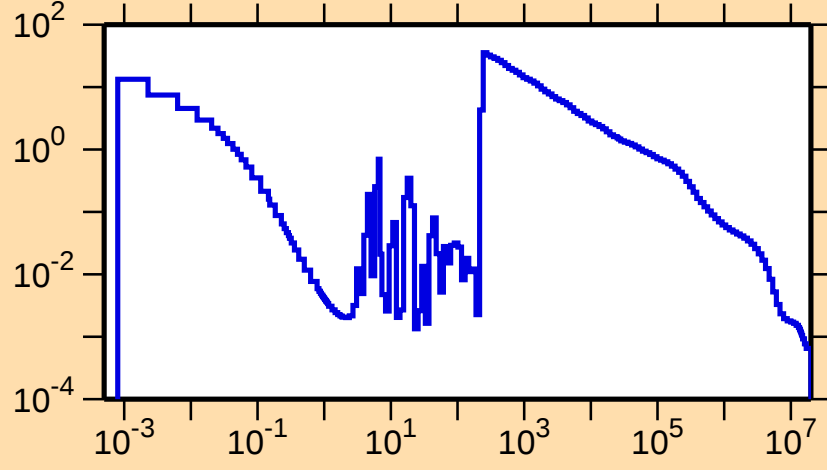
\sigma vs. E for ^{188}\text{Re}(n,\gamma)
