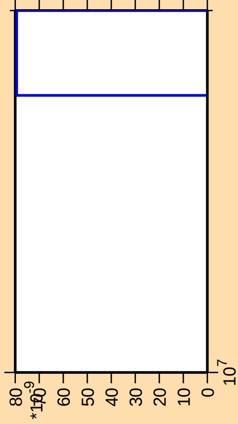
\Delta\sigma/\sigma vs. E for ^{188}\text{Re}(\text{mt } 42)
