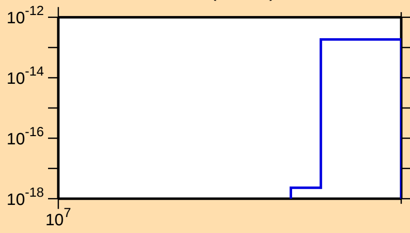
\sigma vs. E for ^{188}\text{Re}(n,3n\alpha)
