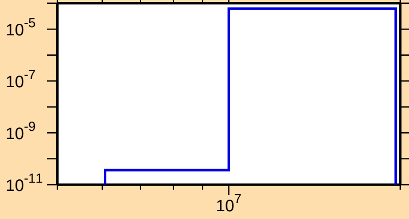
\sigma vs. E for ^{188}\text{Re}(n,t)
