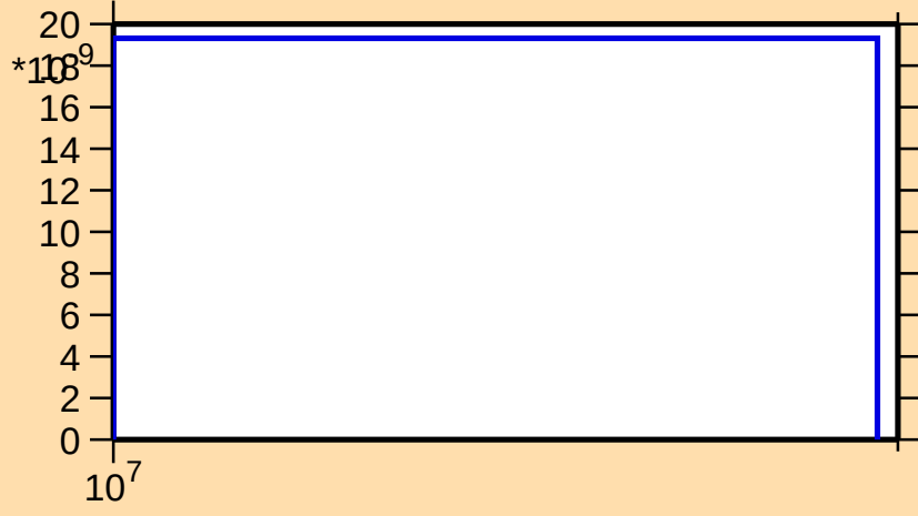
\sigma vs. E for ^{188}\text{Re}(n,nt)
