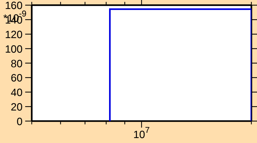
\sigma vs. E for ^{188}\text{Re}(n,\text{nd})
