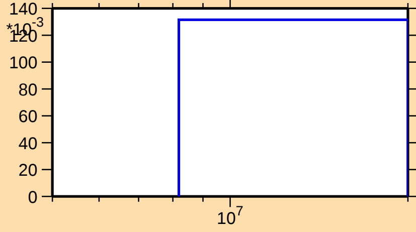
\sigma vs. E for ^{188}\text{Re}(n,3n)
