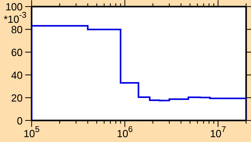
\sigma vs. E for ^{188}\text{Re}(n,n_3)
