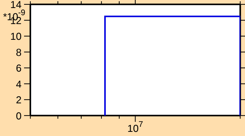
\sigma vs. E for ^{188}\text{Re}(n,2n\alpha)
