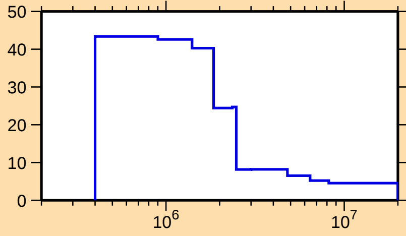
\Delta\sigma/\sigma vs. E for ^{188}\text{Re}(n,n\text{nonel.})
