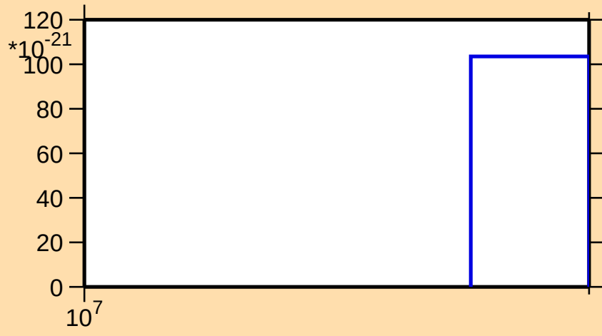
\sigma vs. E for ^{188}\text{Re}(\text{mt } 42)
