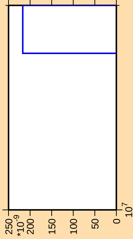
\Delta\sigma/\sigma vs. E for ^{188}\text{Re}(\text{mt } 42)
