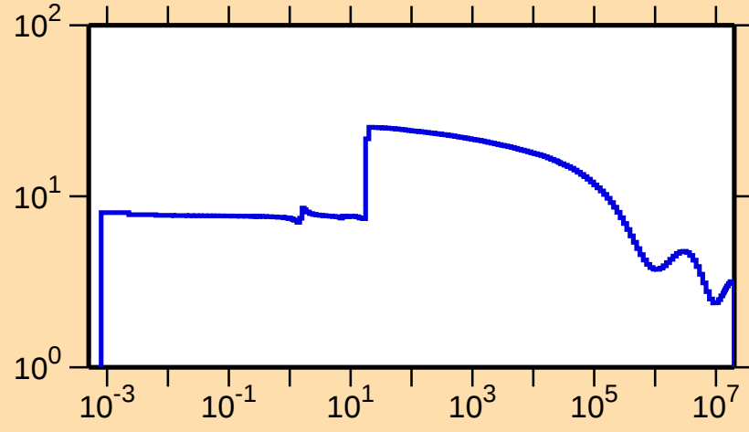
\sigma vs. E for ^{192}\text{Re}(n,\text{el.})
