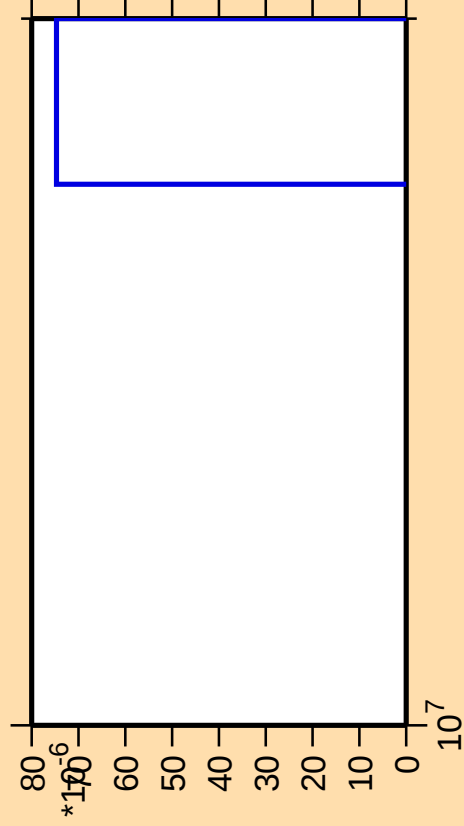
\Delta\sigma/\sigma vs. E for ^{192}\text{Re}(\text{mt } 42)
