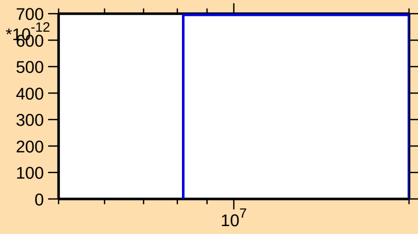
\sigma vs. E for ^{192}\text{Re}(n,2n\alpha)
