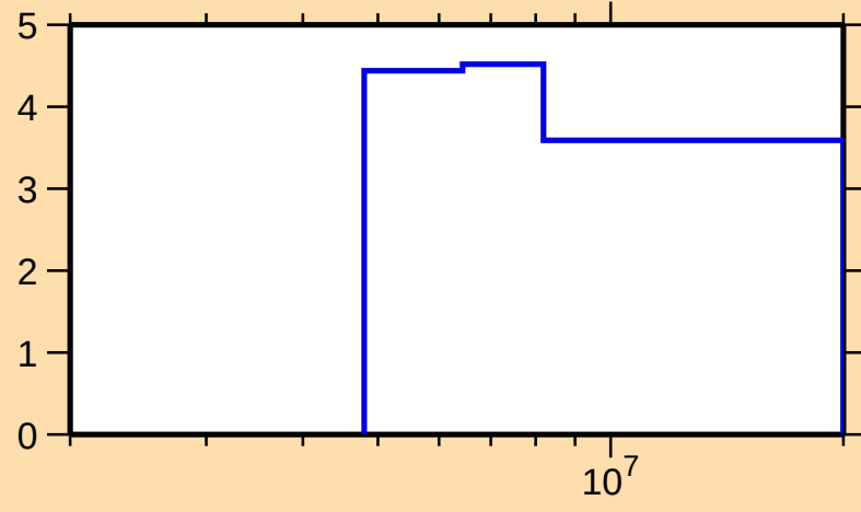
\Delta\sigma/\sigma vs. E for ^{192}\text{Re}(n,\text{nonel.})
