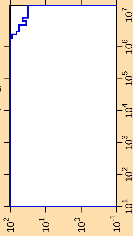
\Delta\sigma/\sigma vs. E for ^{192}\text{Re}(n,n_1)
