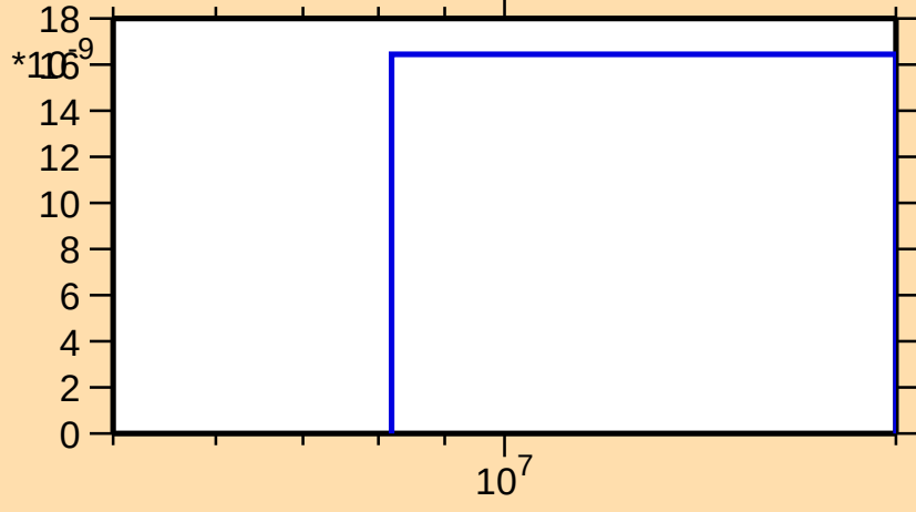
\sigma vs. E for ^{192}\text{Re}(n,nt)
