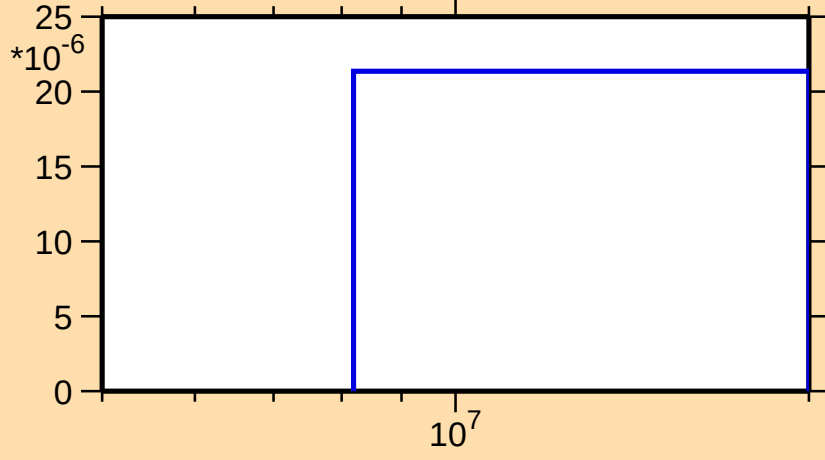
\sigma vs. E for ^{192}\text{Re}(n,t)
