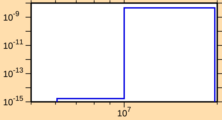
\sigma vs. E for ^{257}\text{He3} )
