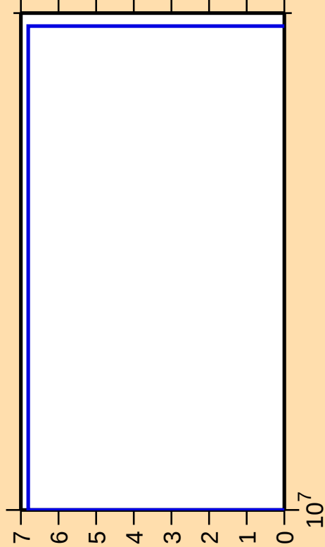
\Delta\sigma/\sigma vs. E for ^{257}
