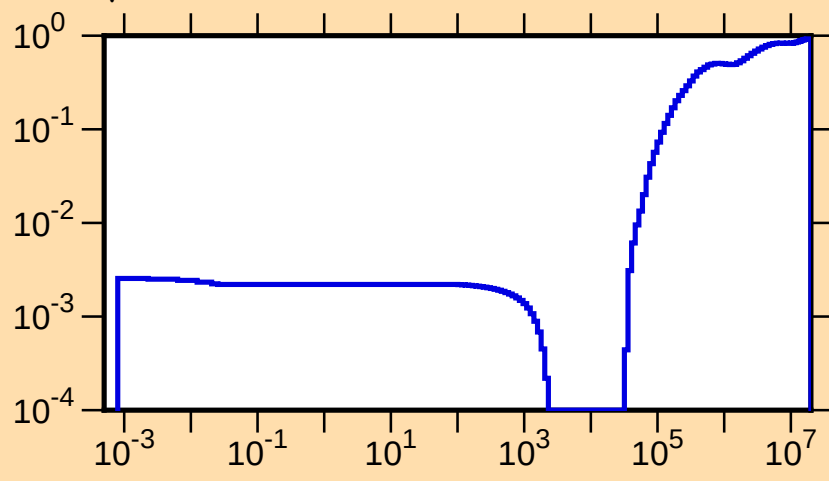
\mu vs. E for ^{261}
