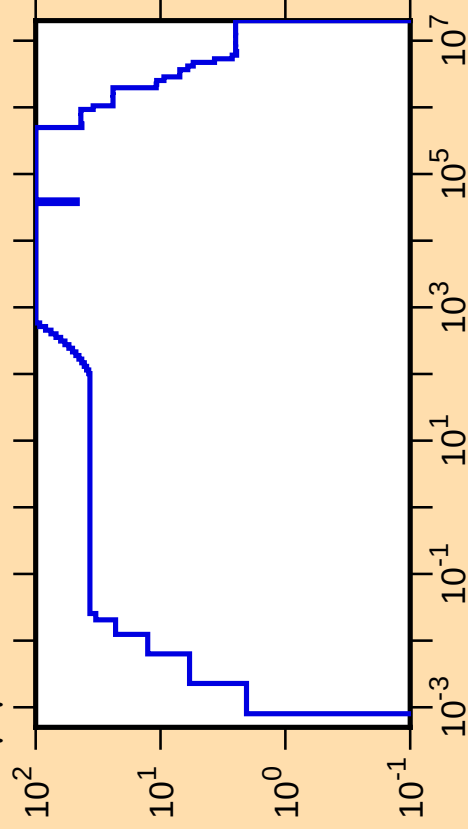
\Delta\mu/\mu vs. E for ^{261}
