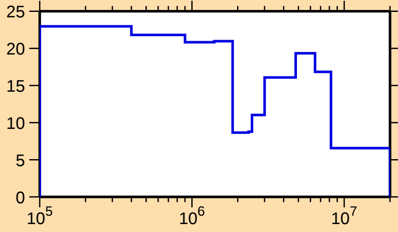
\Delta\sigma/\sigma vs. E for ^{261}\text{I}
