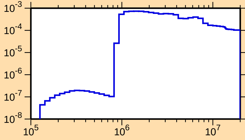
\sigma vs. E for ^{281}
