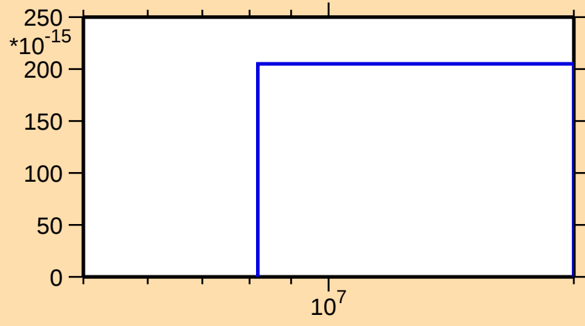
\sigma vs. E for ^{281}\text{He3}
