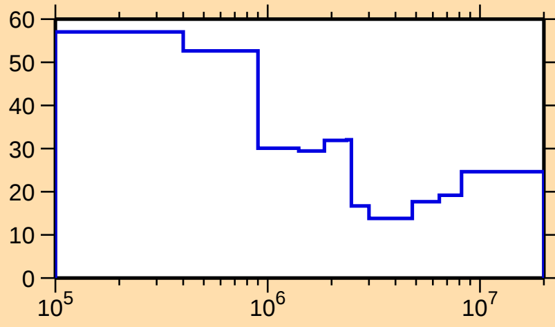
\Delta\sigma/\sigma vs. E for ^{281}\text{I}
