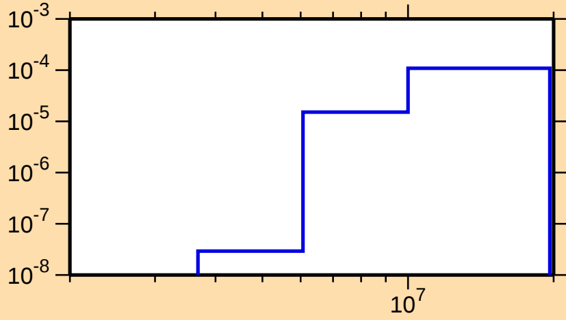
\sigma vs. E for ^{282}\alpha )
