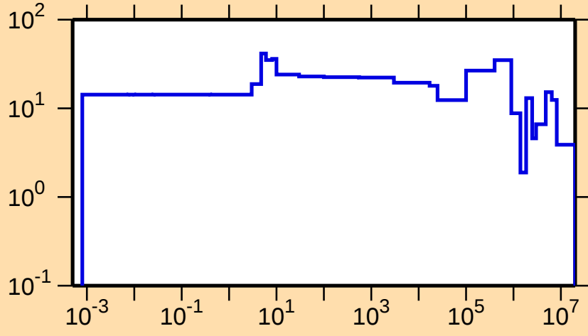
\Delta\sigma/\sigma vs. E for ^{282}
