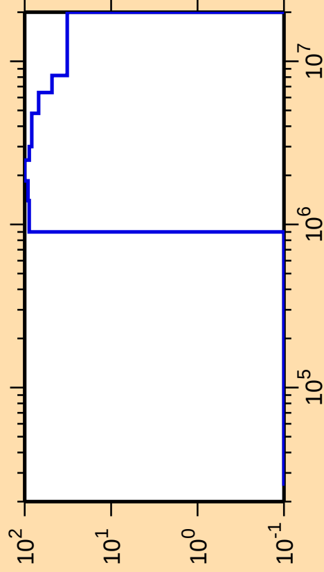
\Delta\sigma/\sigma vs. E for ^{282}_{11}
