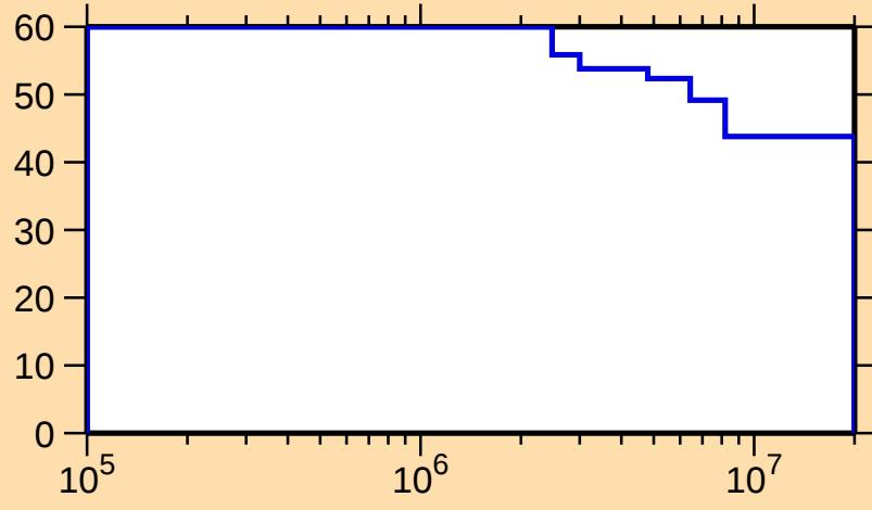
\Delta\sigma/\sigma vs. E for ^{282}
