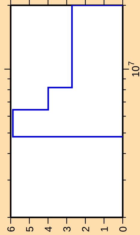
\Delta\sigma/\sigma vs. E for ^{282}
