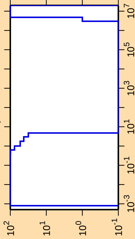
\Delta\sigma/\sigma vs. E for ^{282}\alpha )
