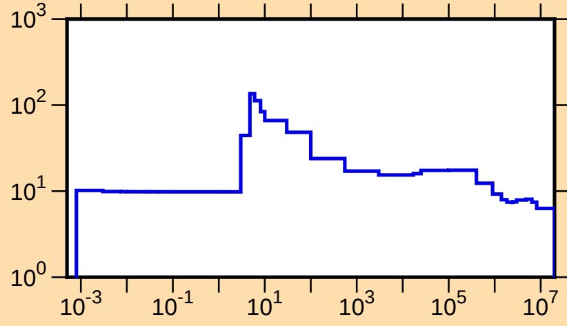
\sigma vs. E for ^{282}
