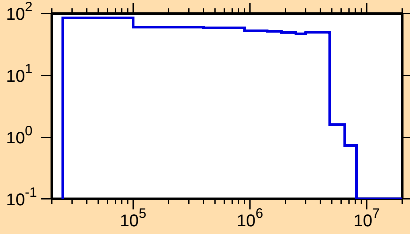
\Delta\sigma/\sigma vs. E for ^{282}_{11}
