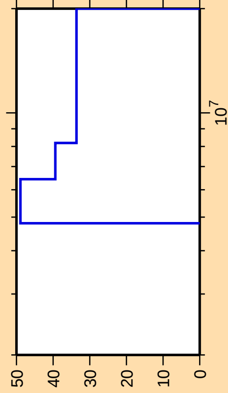
\Delta\sigma/\sigma vs. E for ^{282}
