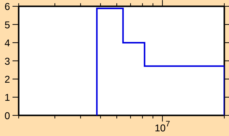
\Delta\sigma/\sigma vs. E for ^{282}
