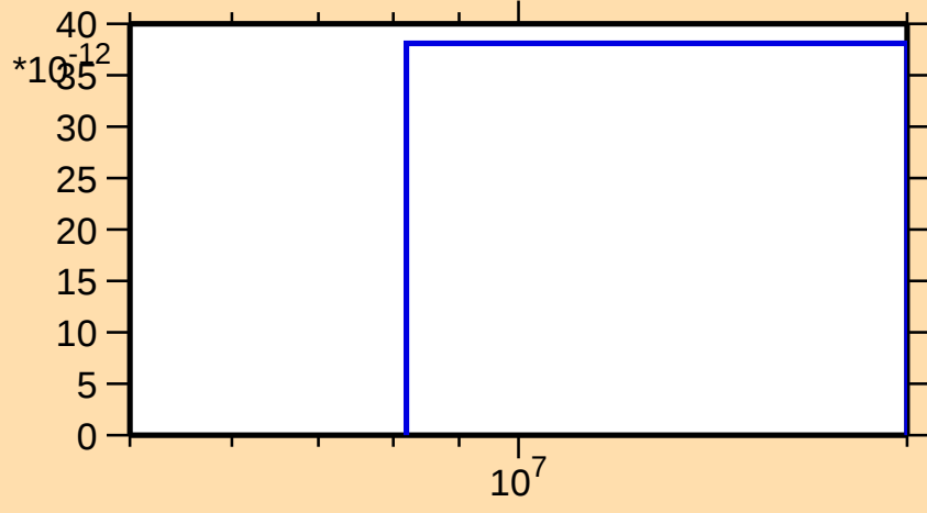
\sigma vs. E for ^{282}\text{He3} )
