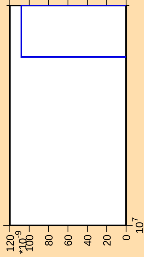
\Delta\sigma/\sigma vs. E for ^{91}\text{Rh}(n,\text{nt})
