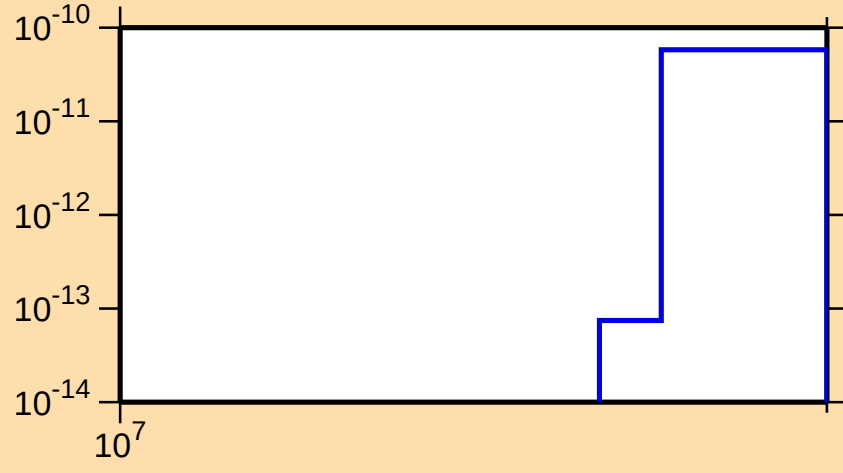
\sigma vs. E for ^{91}\text{Rh}(\text{mt } 34)
