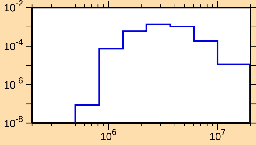
\sigma vs. E for ^{91}\text{Rh}(n,n\text{cont.})
