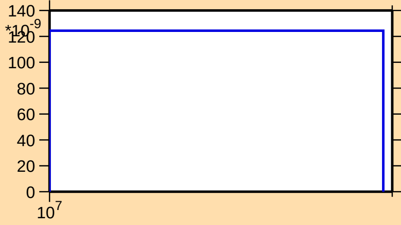
\sigma vs. E for ^{91}\text{Rh}(n,\text{pt})
