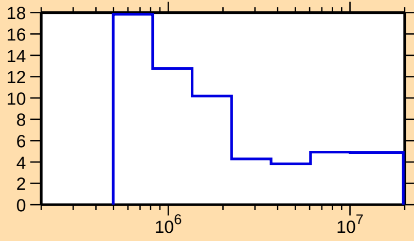
\Delta\sigma/\sigma vs. E for ^{91}\text{Rh}(n,\text{nonel.})
