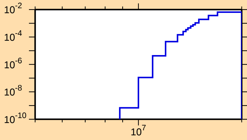
\sigma vs. E for ^{93}\text{Rh}(n,\text{pd})
