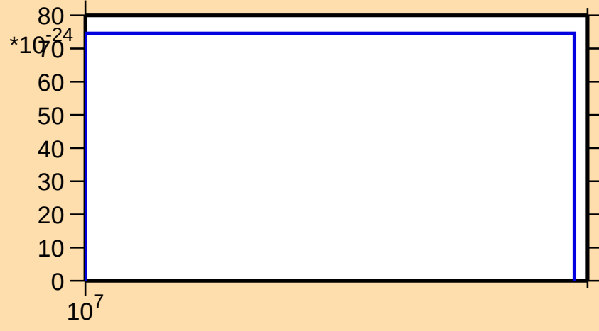
\sigma vs. E for ^{93}\text{Rh}(n,\text{nt})
