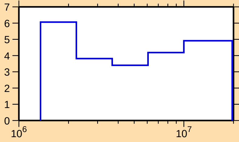
\Delta\sigma/\sigma vs. E for ^{93}\text{Rh}(n,n\text{oncl.})
