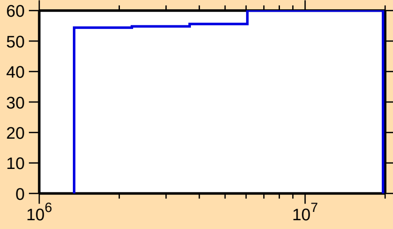
\Delta\sigma/\sigma vs. E for ^{93}\text{Rh}(n,n\text{cont.})
