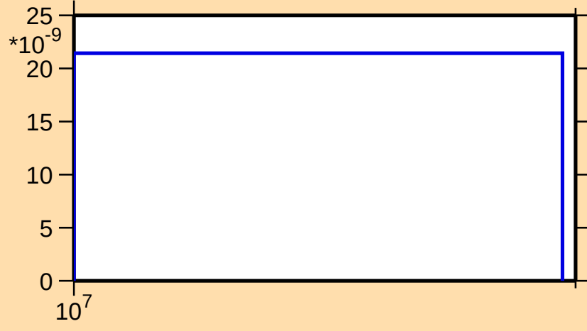
\sigma vs. E for ^{93}\text{Rh}(\text{mt } 45)
