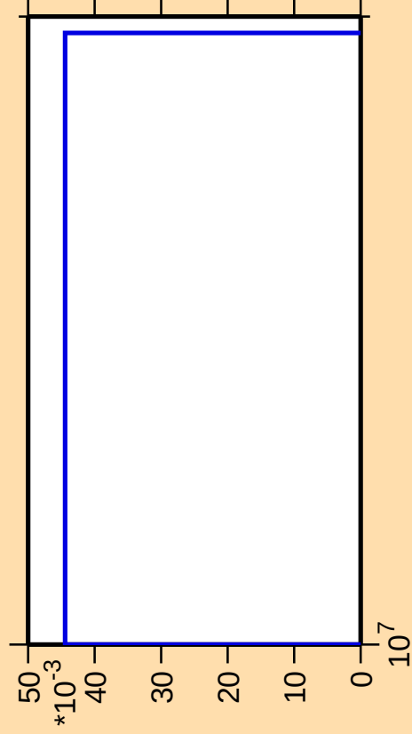
\Delta\sigma/\sigma vs. E for ^{93}\text{Rh}(\text{mt } 34)
