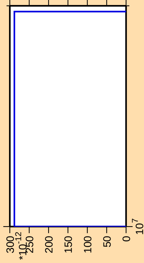
\Delta\sigma/\sigma vs. E for ^{93}\text{Rh}(n,\text{nt})
