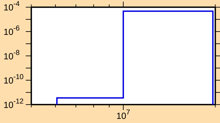
\sigma vs. E for ^{93}\text{Rh}(n,n\alpha)
