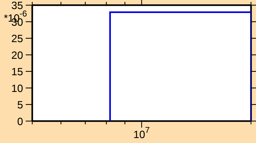
\sigma vs. E for ^{93}\text{Rh}(n,2n)
