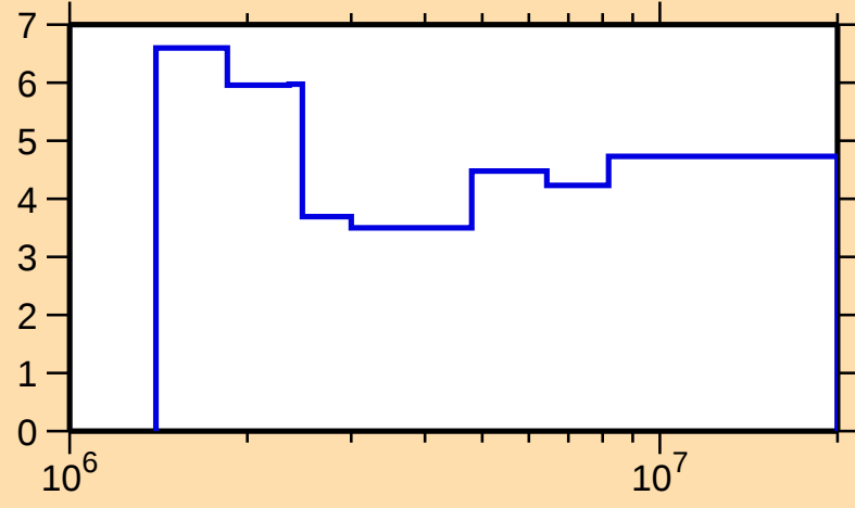
\Delta\sigma/\sigma vs. E for ^{93}\text{Rh}(n,n\text{nonel.})
