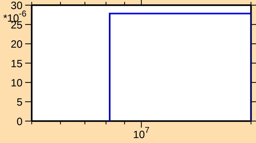
\sigma vs. E for ^{93}\text{Rh}(n,t)
