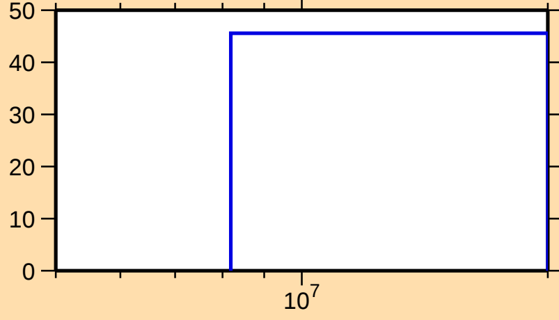
\Delta\sigma/\sigma vs. E for ^{93}\text{Rh}(n,2n)
