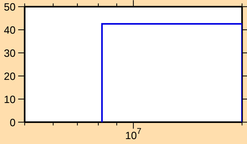
\Delta\sigma/\sigma vs. E for ^{93}\text{Rh}(n,\text{inel.})
