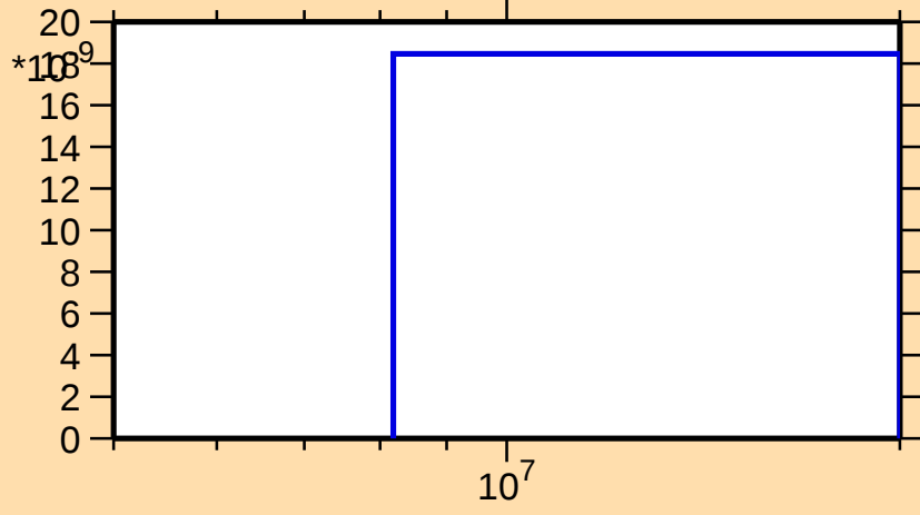
\sigma vs. E for ^{93}\text{Rh}(\text{mt 45})
