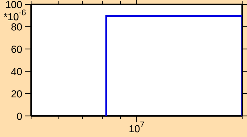
\sigma vs. E for ^{106}\text{Rh}(n,n\alpha)
