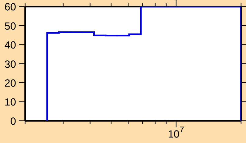
\Delta\sigma/\sigma vs. E for ^{110}\text{Rh}(n,n\text{cont.})
