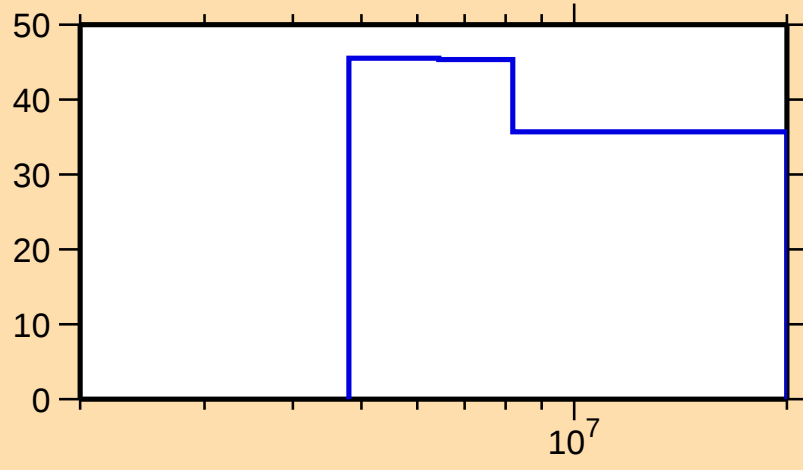
\Delta\sigma/\sigma vs. E for ^{110}\text{Rh}(n,2n)
