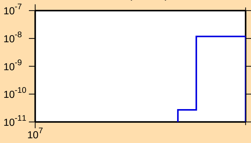
\sigma vs. E for ^{110}\text{Rh}(n,2n\alpha)
