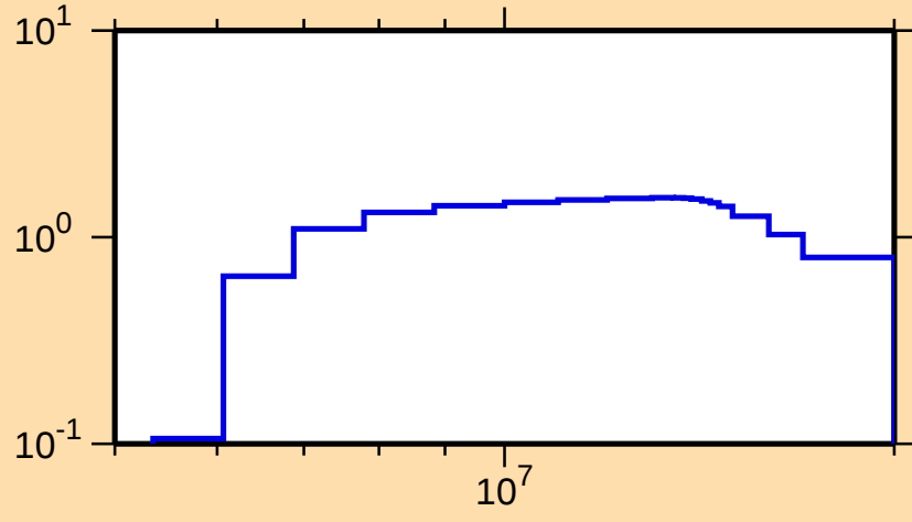
\sigma vs. E for ^{112}\text{Rh}(n,2n)
