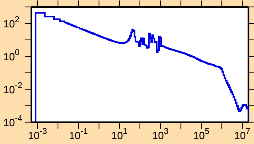
\sigma vs. E for ^{114}\text{Rh}(n,\gamma)
