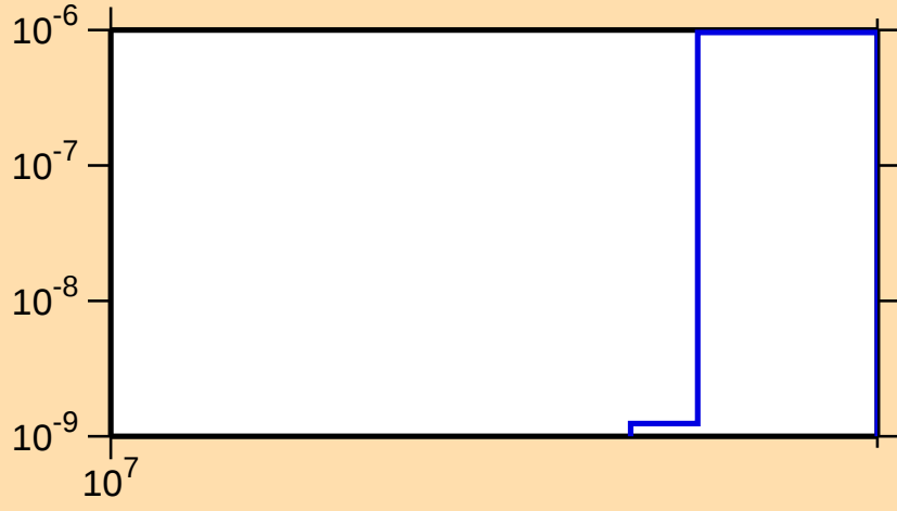
\sigma vs. E for ^{114}\text{Rh}(n,\text{nt})
