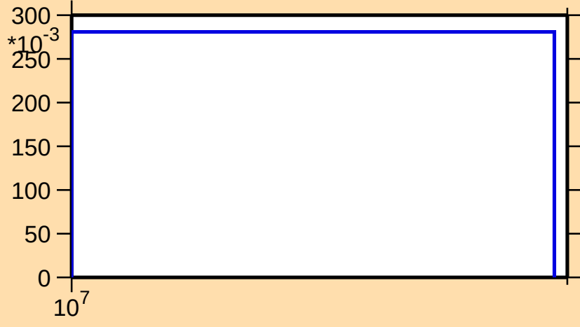
\sigma vs. E for ^{114}\text{Rh}(n,3n)
