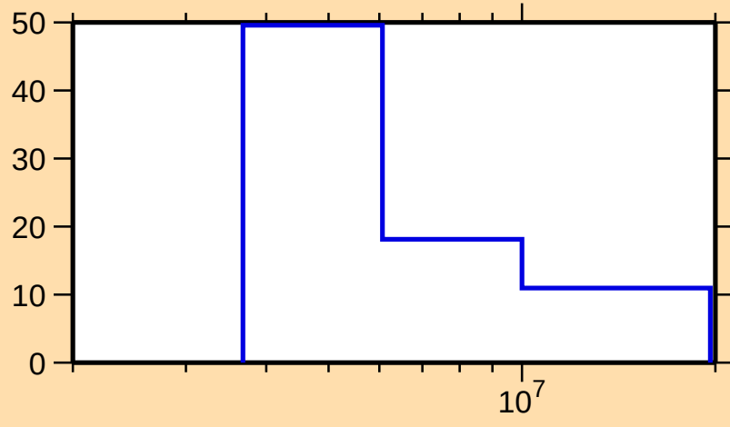
\Delta\sigma/\sigma vs. E for ^{114}\text{Rh}(n,\text{el.})
