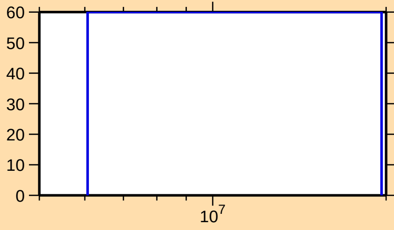
\Delta\sigma/\sigma vs. E for ^{114}\text{Rh}(n,n\text{cont.})
