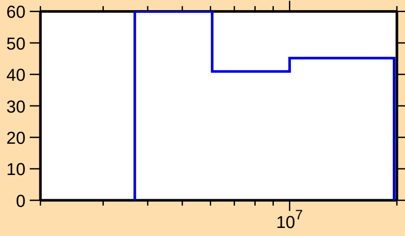
\Delta\sigma/\sigma vs. E for ^{114}\text{Rh}(n,2n)
