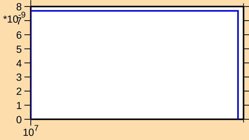
\sigma vs. E for ^{114}\text{Rh}(n,nt)
