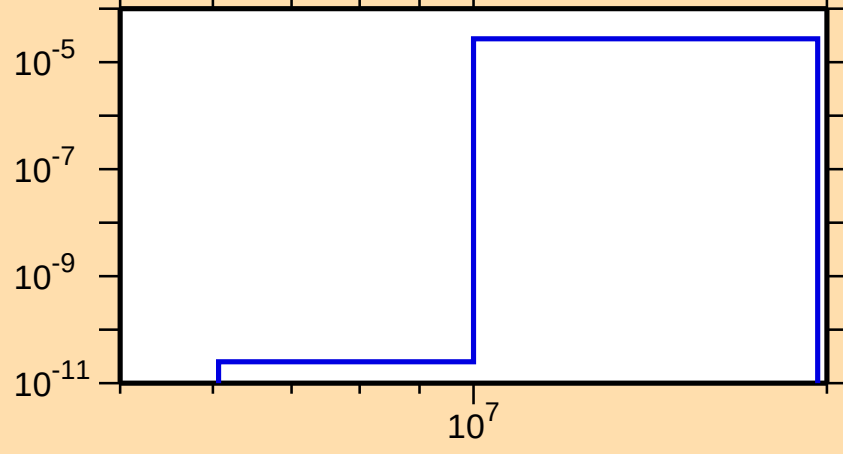
\sigma vs. E for ^{114}\text{Rh}(n,\alpha)
