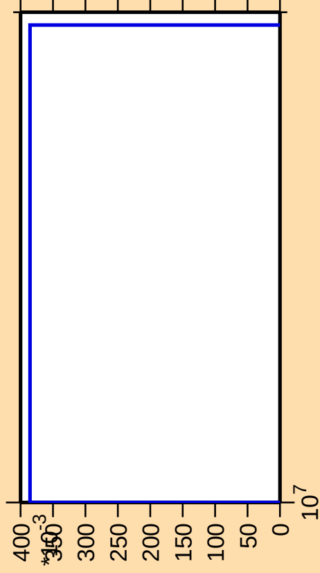
\Delta\sigma/\sigma vs. E for ^{114}\text{Rh}(n,2n\alpha)
