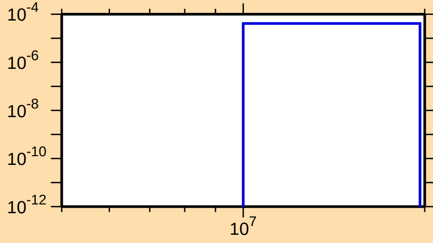
\sigma vs. E for ^{114}\text{Rh}(n,d)
