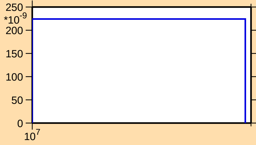
\sigma vs. E for ^{114}\text{Rh}(n,n\alpha)
