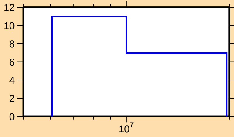
\Delta\sigma/\sigma vs. E for ^{114}\text{Rh}(n,\text{tot.})
