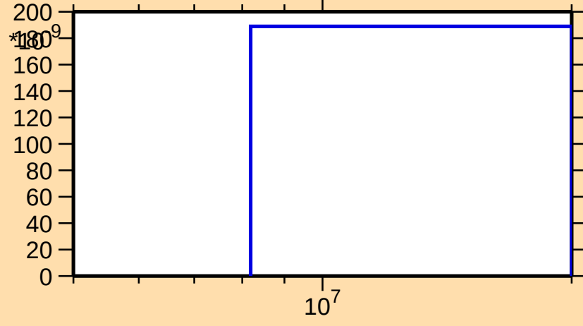
\sigma vs. E for ^{114}\text{Rh}(n,n\alpha)
