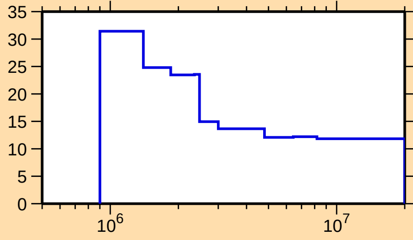
\Delta\sigma/\sigma vs. E for ^{114}\text{Rh}(n,n\text{onel.})
