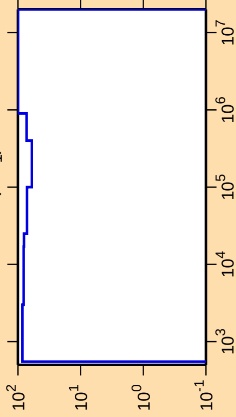
\Delta\sigma/\sigma vs. E for ^{114}\text{Rh}(n,n_1)
