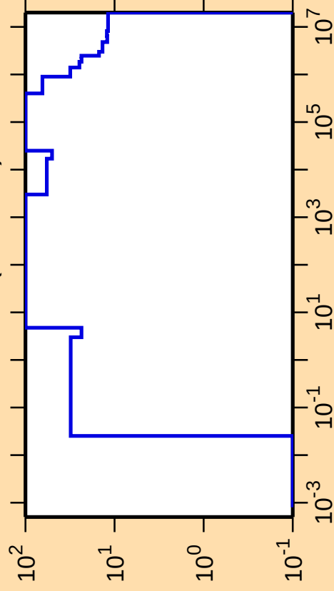
\Delta\sigma/\sigma vs. E for ^{114}\text{Rh}(n,\text{nonel.})
