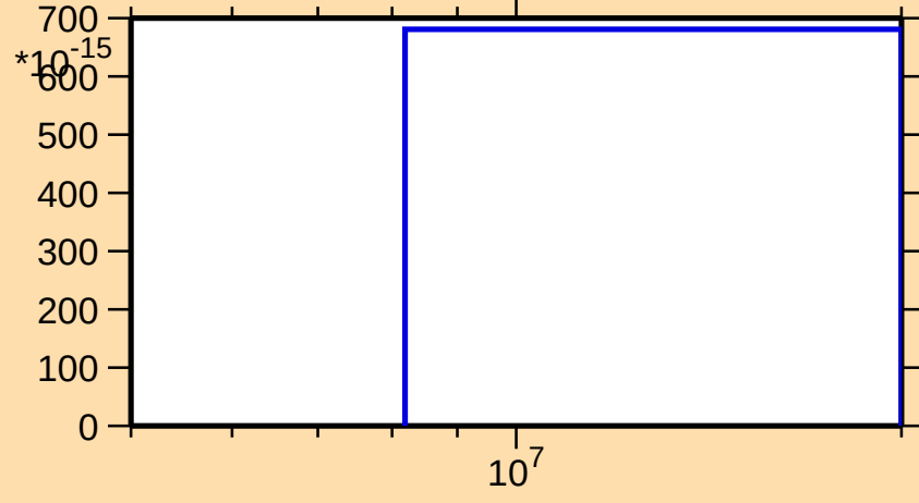
\sigma vs. E for ^{114}\text{Rh}(n,2n\alpha)
