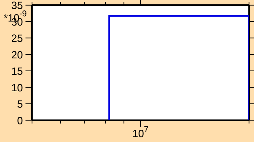
\sigma vs. E for ^{114}\text{Rh}(n,\text{nd})
