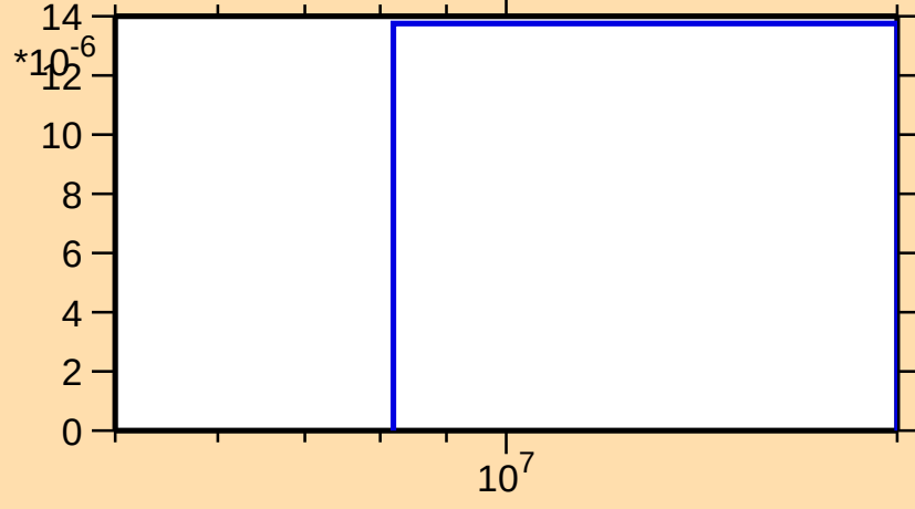
\sigma vs. E for ^{114}\text{Rh}(n,np)
