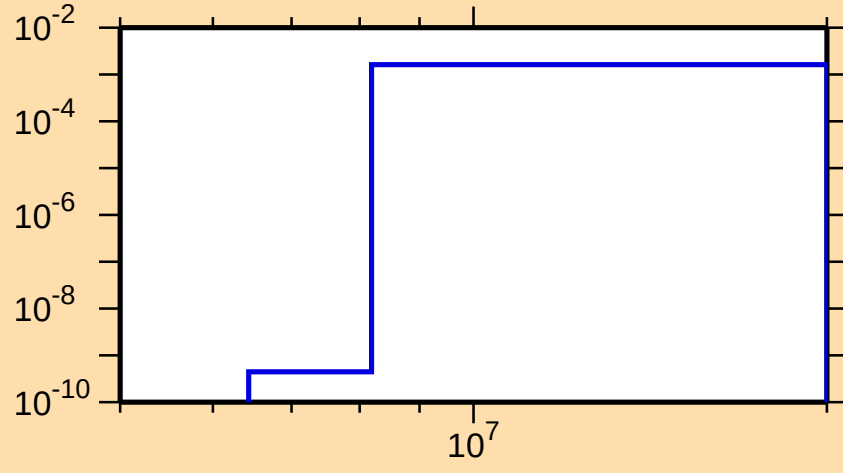
\sigma vs. E for ^{114}\text{Rh}(n,p)
