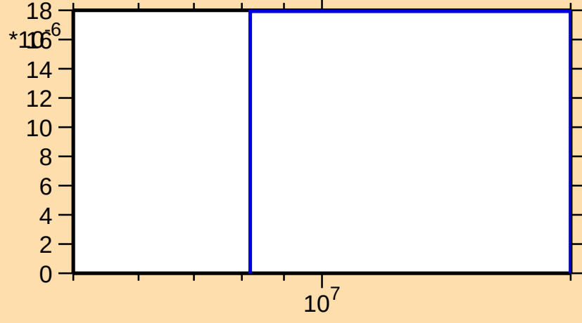
\sigma vs. E for ^{114}\text{Rh}(n,t)
