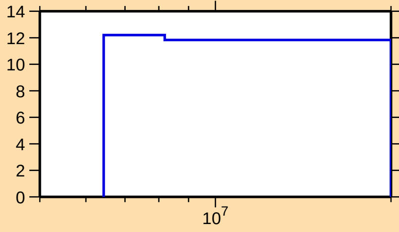
\Delta\sigma/\sigma vs. E for ^{114}\text{Rh}(n,\text{nonel.})
