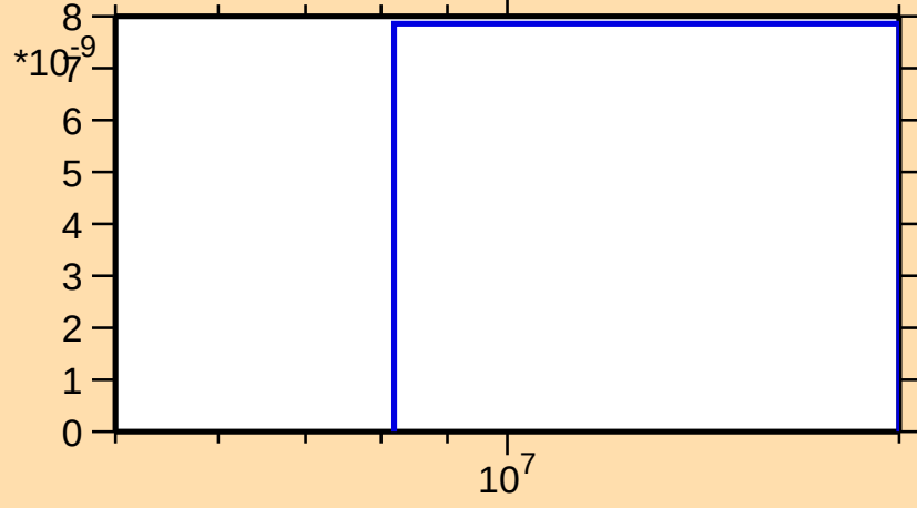
\sigma vs. E for ^{114}\text{Rh}(n,nt)
