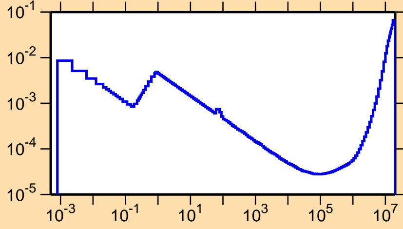
\sigma vs. E for ^{200}\text{Rn}(n,\alpha)
