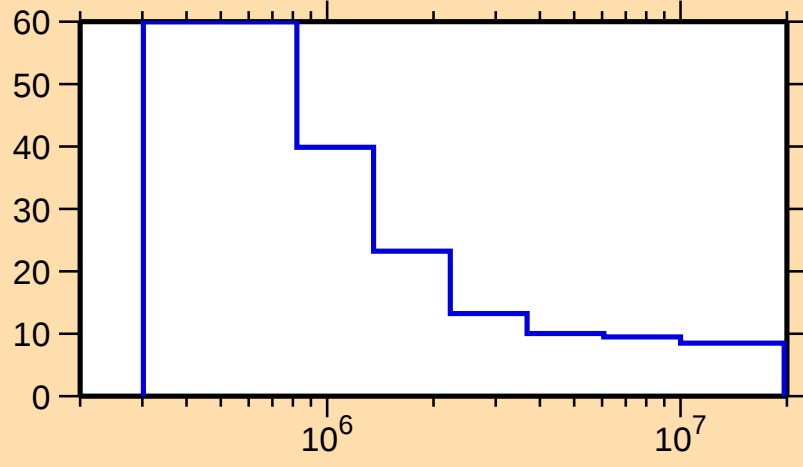
\Delta\sigma/\sigma vs. E for ^{200}\text{Rn}(n,\text{nonel.})
