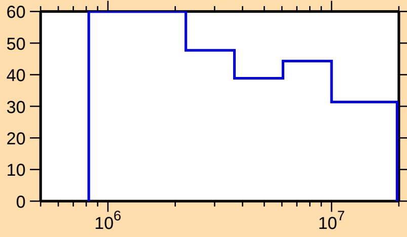
\Delta\sigma/\sigma vs. E for ^{200}\text{Rn}(n,n_1)
