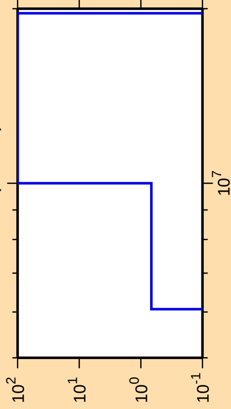
\Delta\sigma/\sigma vs. E for ^{200}\text{Rn}(\text{mt117})
