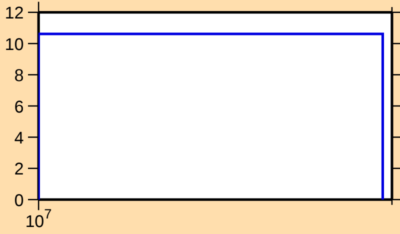
\Delta\sigma/\sigma vs. E for ^{200}\text{Rn}(n,\text{el.})
