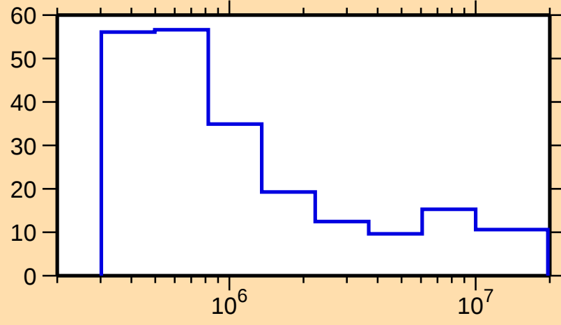
\Delta\sigma/\sigma vs. E for ^{200}\text{Rn}(n,\text{el.})
