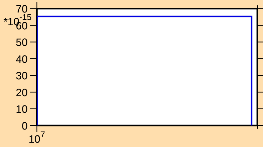
\sigma vs. E for ^{200}\text{Rn}(\text{mt } 34)
