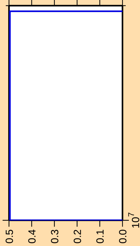
\Delta\sigma/\sigma vs. E for ^{200}\text{Rn}(\text{mt } 34)
