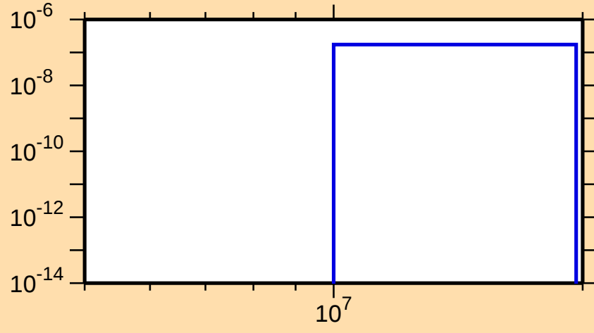
\sigma vs. E for ^{200}\text{Rn}(n,2n\alpha)
