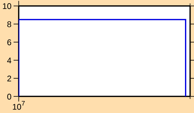
\Delta\sigma/\sigma vs. E for ^{200}\text{Rn}(n,\text{nonel.})
