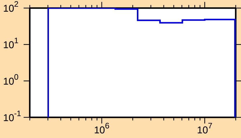
\Delta\sigma/\sigma vs. E for ^{200}\text{Rn}(n,\text{inel.})
