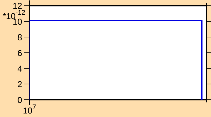
\sigma vs. E for ^{200}\text{Rn}(n,\text{pt})
