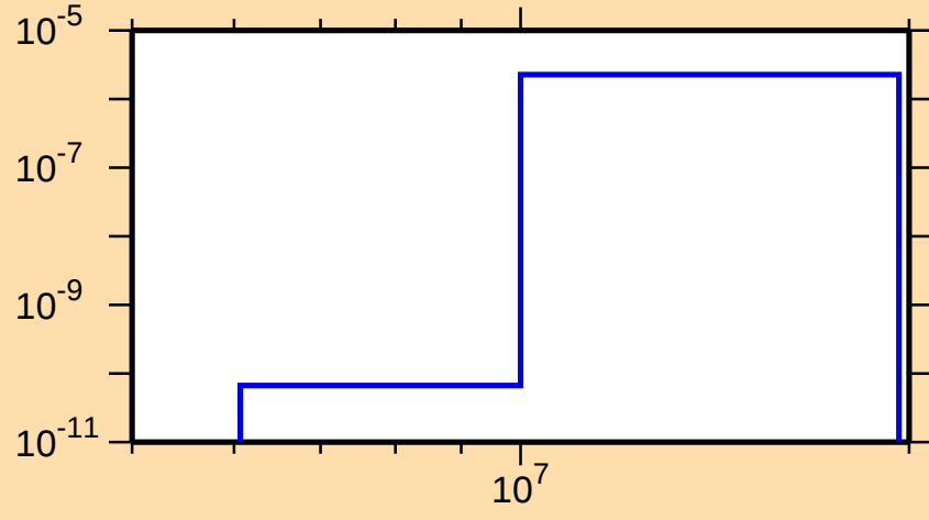
\sigma vs. E for ^{200}\text{Rn}(n,\text{He}3)
