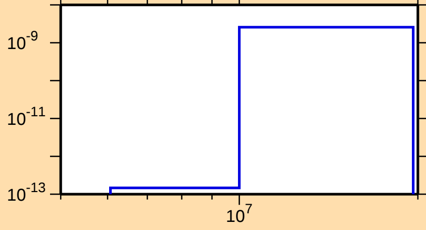
\sigma vs. E for ^{200}\text{Rn}(\text{mt117})
