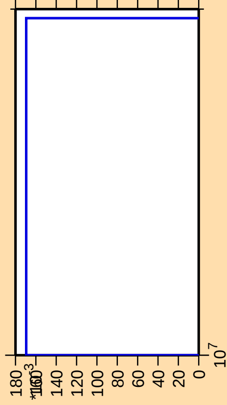
\Delta\sigma/\sigma vs. E for ^{200}\text{Rn}(n,nt)
