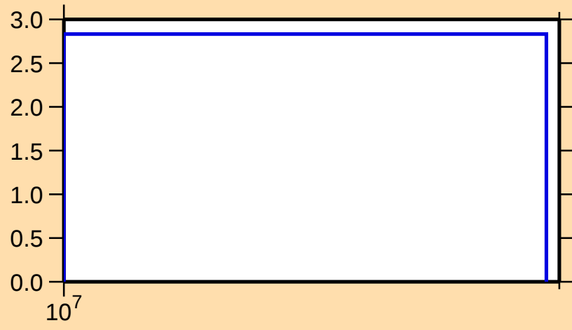
\Delta\sigma/\sigma vs. E for ^{200}\text{Rn}(n,\text{tot.})
