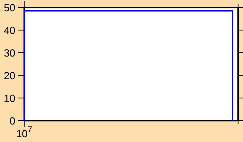
\Delta\sigma/\sigma vs. E for ^{200}\text{Rn}(n,\text{inel.})
