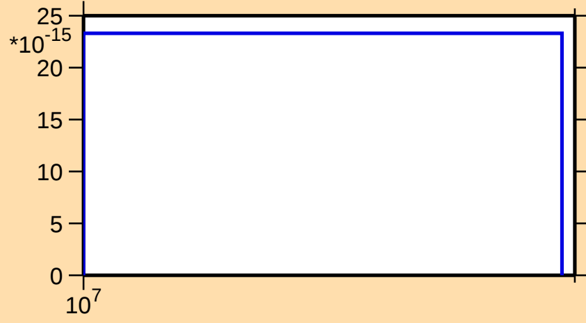
\sigma vs. E for ^{200}\text{Rn}(n,nt)
