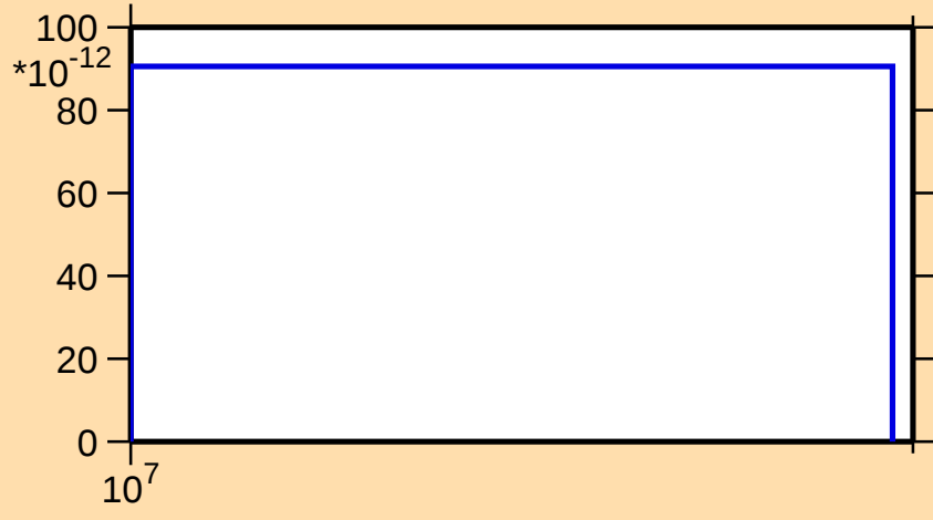
\sigma vs. E for ^{200}\text{Rn}(n,\text{nd})
