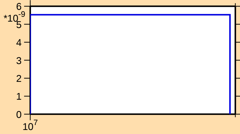
\sigma vs. E for ^{200}\text{Rn}(n,2np)
