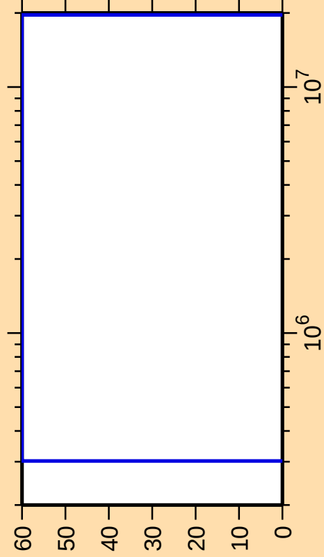
\Delta\sigma/\sigma vs. E for ^{200}\text{Rn}(n,p)
