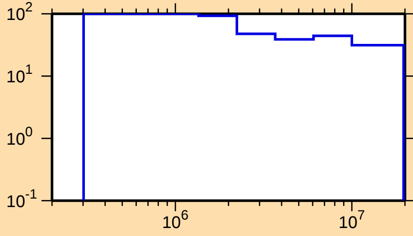
\Delta\sigma/\sigma vs. E for ^{200}\text{Rn}(n,n_1)
