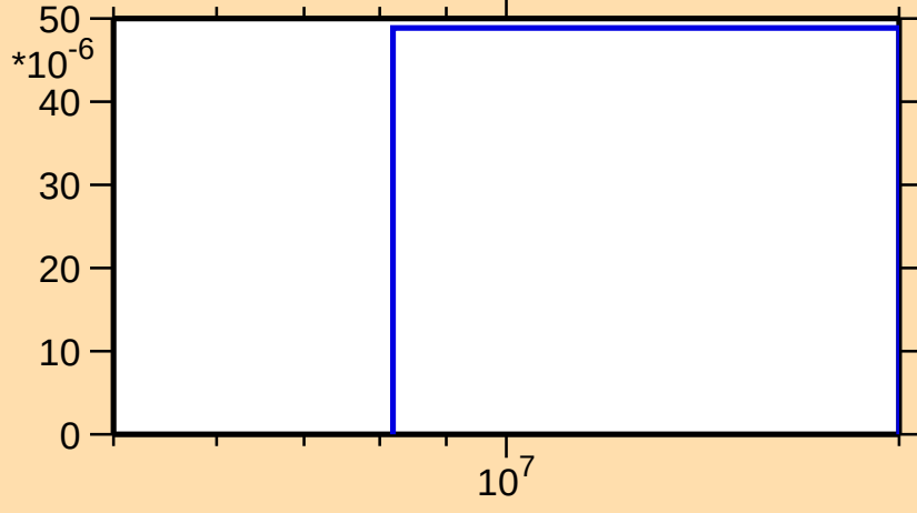
\sigma vs. E for ^{200}\text{Rn}(n,t)
