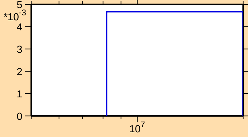
\sigma vs. E for ^{200}\text{Rn}(n,2n)
