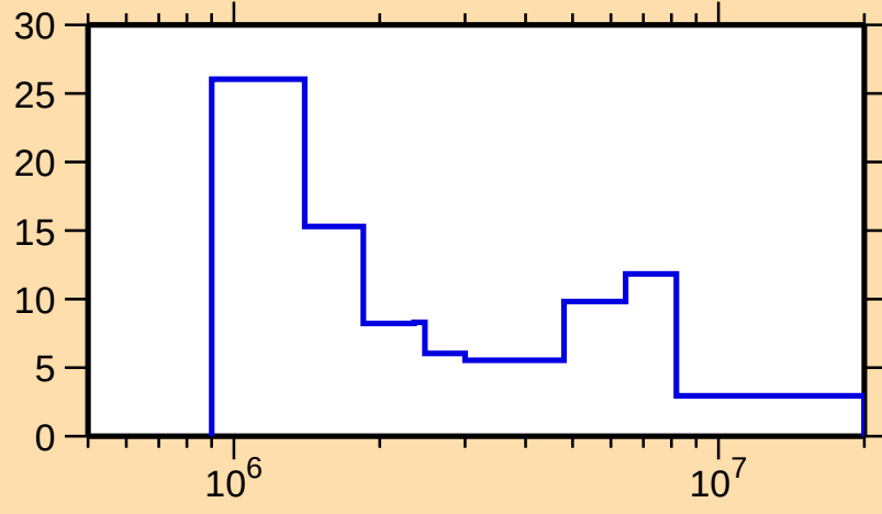
\Delta\sigma/\sigma vs. E for ^{200}\text{Rn}(n,\text{tot.})
