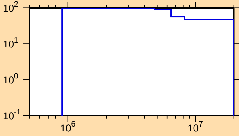
\Delta\sigma/\sigma vs. E for ^{200}\text{Rn}(n,n\text{cont.})
