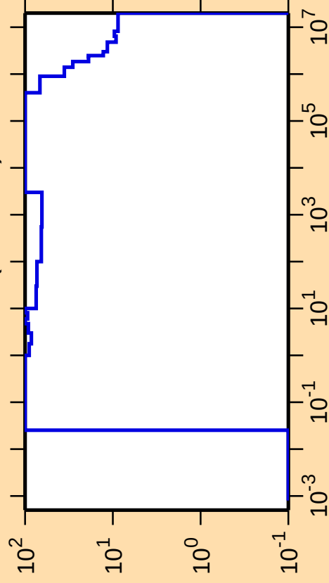
\Delta\sigma/\sigma vs. E for ^{200}\text{Rn}(n,\text{nonel.})
