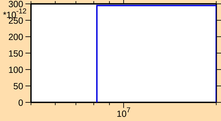
\sigma vs. E for ^{200}\text{Rn}(n,3n)
