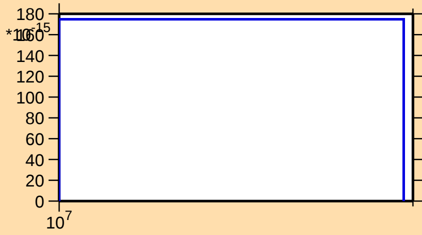
\sigma vs. E for ^{208}\text{Rn}(\text{mt } 34)
