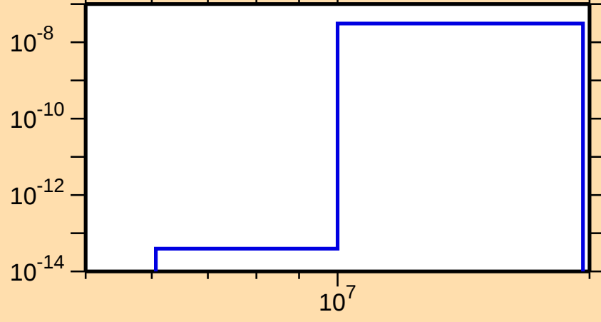
\sigma vs. E for ^{208}\text{Rn}(n,\text{He3})
