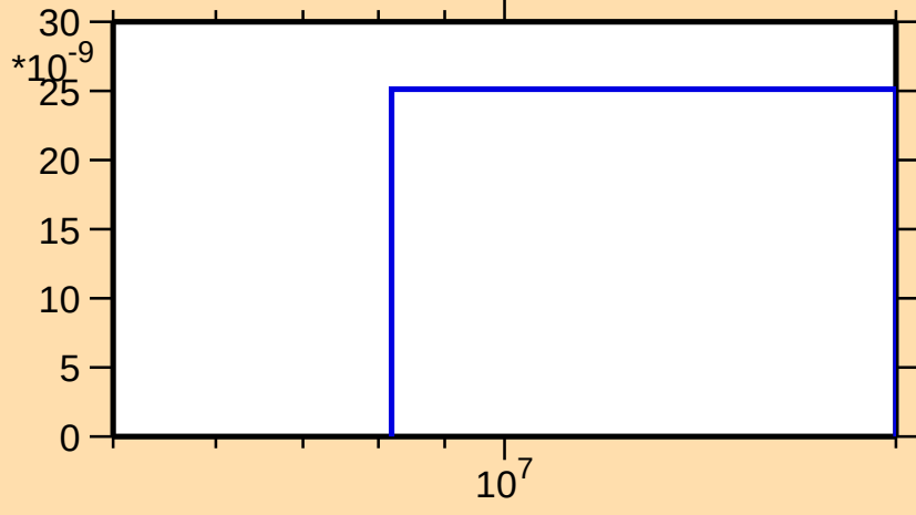
\sigma vs. E for ^{208}\text{Rn}(n,\text{He3})
