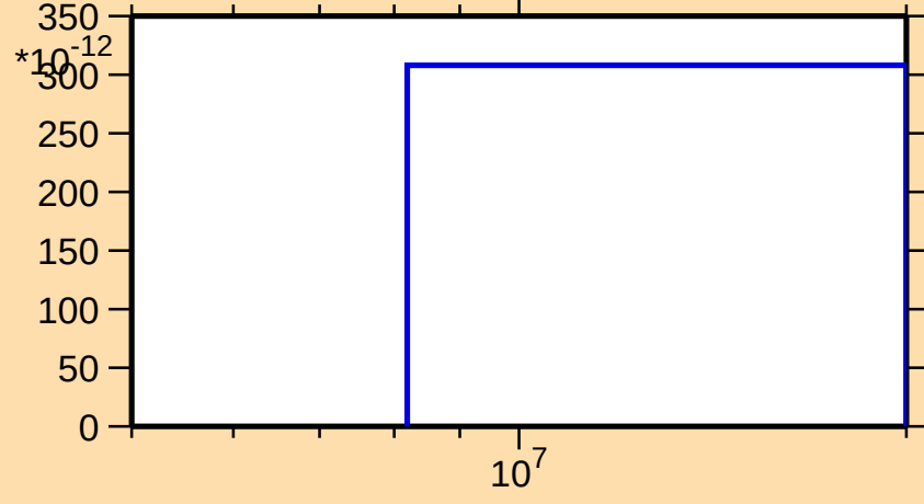
\sigma vs. E for ^{208}\text{Rn}(n,\text{pd})
