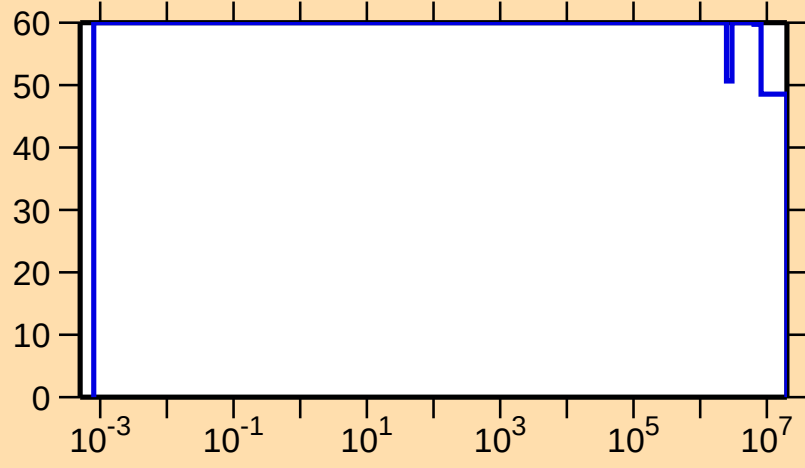
\Delta\sigma/\sigma vs. E for ^{208}\text{Rn}(n,p)
