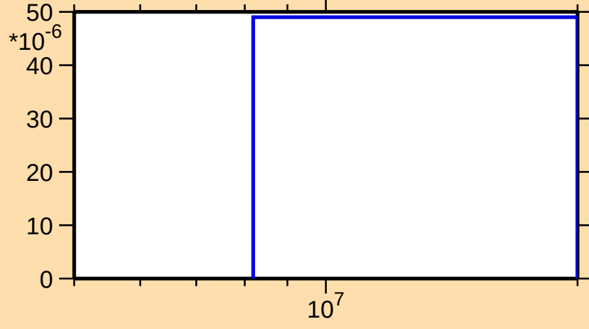
\sigma vs. E for ^{208}\text{Rn}(n,3n)
