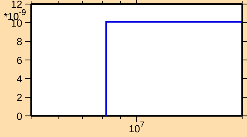
\sigma vs. E for ^{208}\text{Rn}(n,nd)
