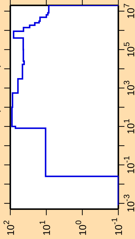
\Delta\sigma/\sigma vs. E for ^{208}\text{Rn}(n,\text{nonel.})
