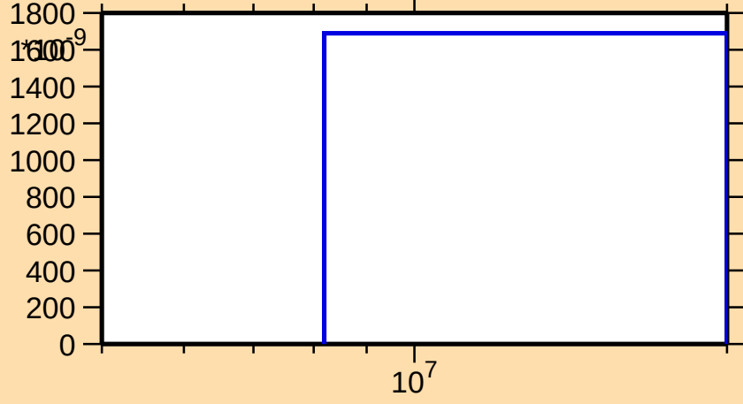
\sigma vs. E for ^{208}\text{Rn}(n,2n\alpha)
