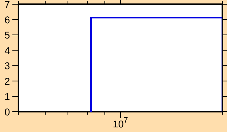
\Delta\sigma/\sigma vs. E for ^{208}\text{Rn}(n,2n)
