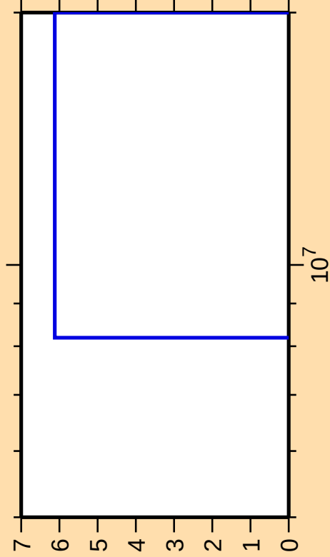
\Delta\sigma/\sigma vs. E for ^{208}\text{Rn}(n,2n)
