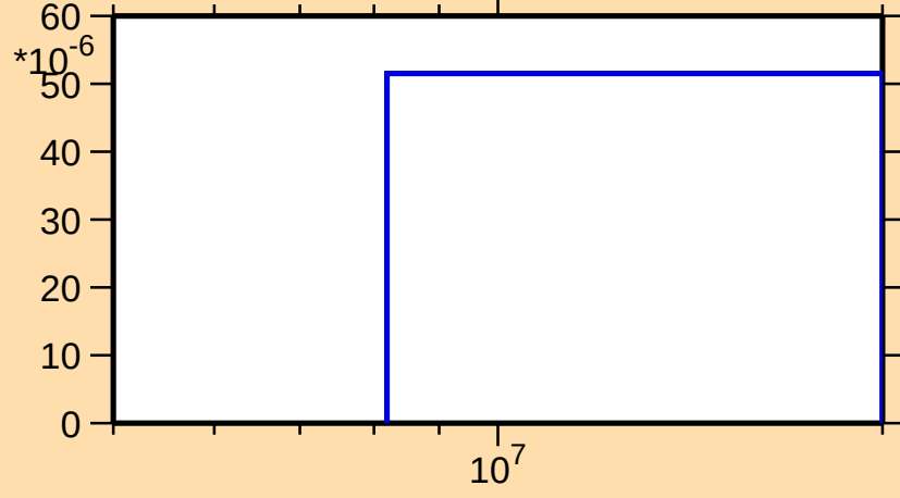
\sigma vs. E for ^{208}\text{Rn}(n,t)
