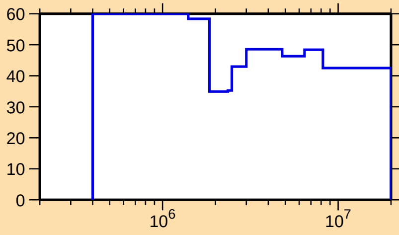
\Delta\sigma/\sigma vs. E for ^{208}\text{Rn}(n,n_1)
