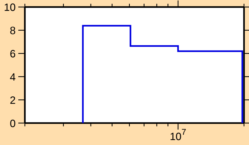
\Delta\sigma/\sigma vs. E for ^{212}\text{Rn}(n,n\text{onel.})
