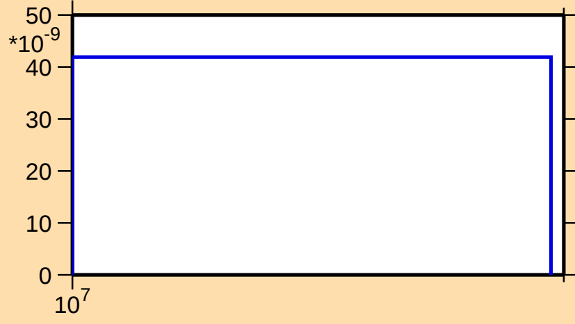
\sigma vs. E for ^{212}\text{Rn}(n,\text{nd})
