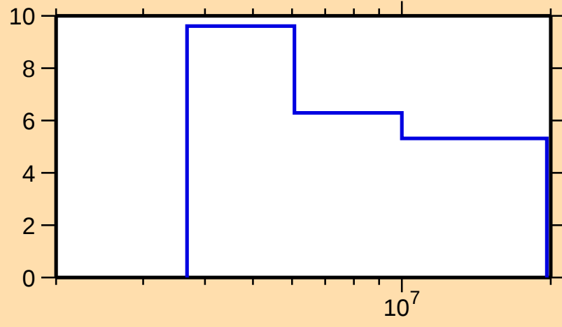
\Delta\sigma/\sigma vs. E for ^{212}\text{Rn}(n,\text{tot.})
