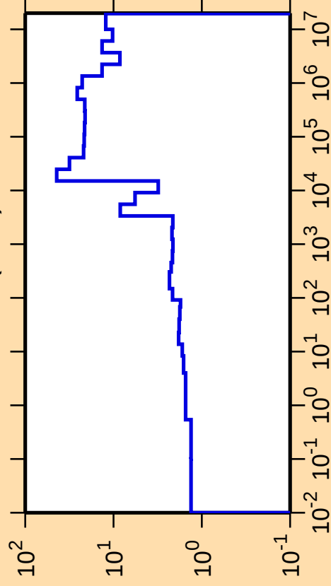
\Delta\sigma/\sigma vs. E for ^{212}\text{Rn}(n,\text{el.})
