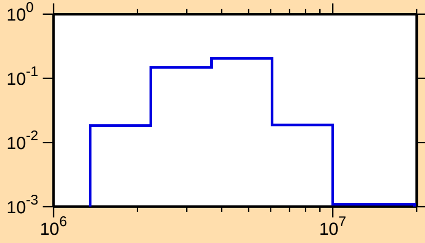
\sigma vs. E for ^{212}\text{Rn}(n,n_3)
