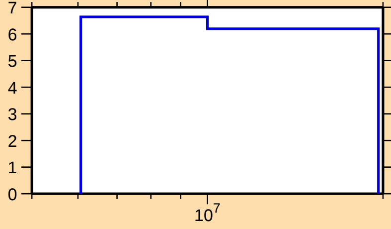
\Delta\sigma/\sigma vs. E for ^{212}\text{Rn}(n,\text{nonel.})
