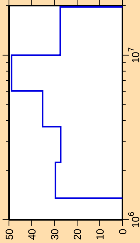
\Delta\sigma/\sigma vs. E for ^{212}\text{Rn}(n,n_3)
