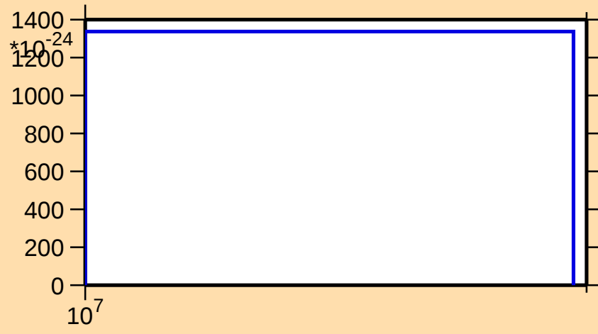
\sigma vs. E for ^{212}\text{Rn}(\text{mt } 42)
