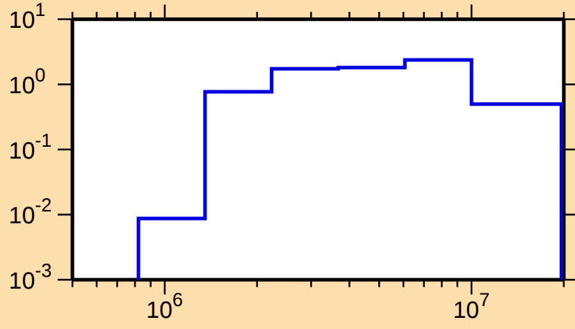
\sigma vs. E for ^{212}\text{Rn}(n,\text{inel.})
