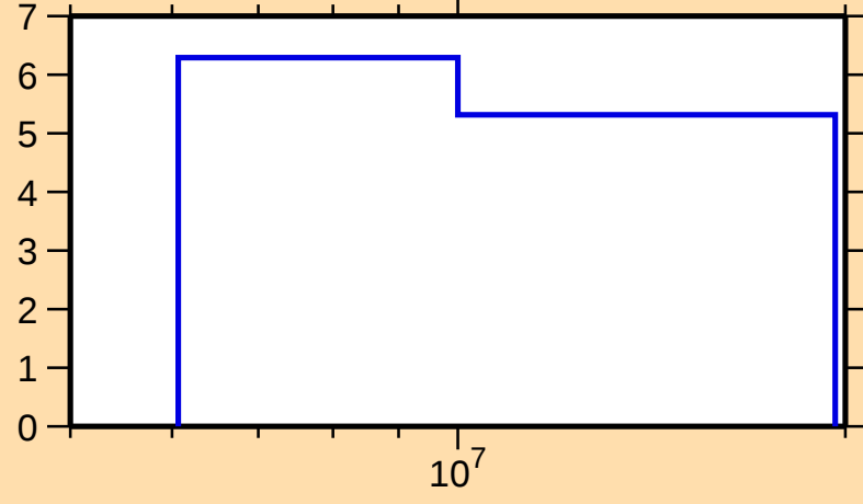
\Delta\sigma/\sigma vs. E for ^{212}\text{Rn}(n,\text{tot.})
