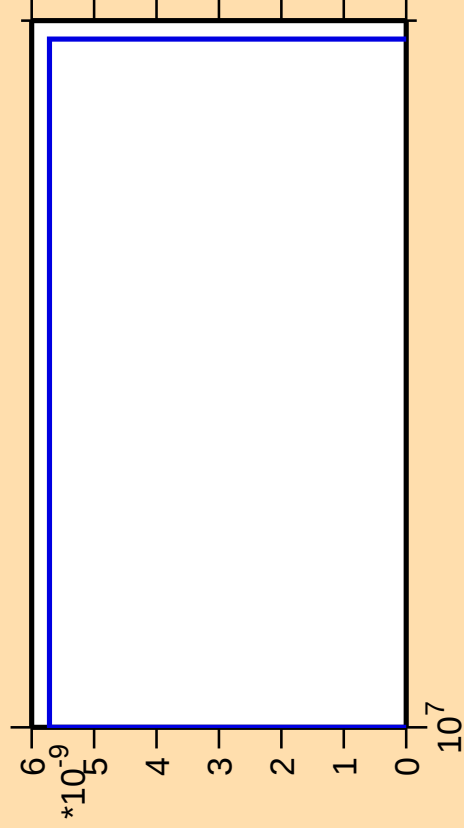
\Delta\sigma/\sigma vs. E for ^{212}\text{Rn}(\text{mt } 42)
