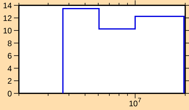
\Delta\sigma/\sigma vs. E for ^{212}\text{Rn}(n,\text{el.})
