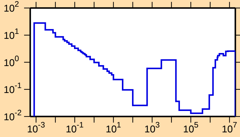
\sigma vs. E for ^{212}\text{Rn}(n,\text{nonel.})
