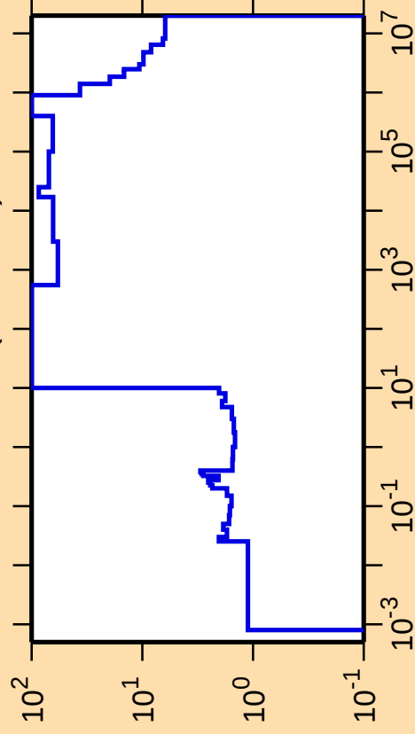
\Delta\sigma/\sigma vs. E for ^{212}\text{Rn}(n,\text{nonel.})
