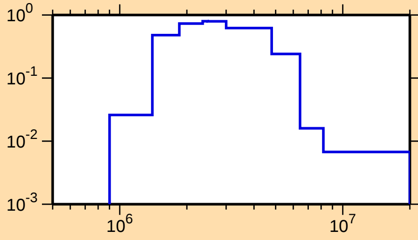
\sigma vs. E for ^{212}\text{Rn}(n,n_1)
