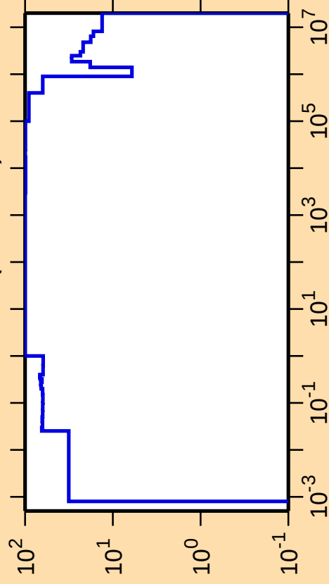
\Delta\sigma/\sigma vs. E for ^{219}\text{Rn}(n,\text{nonel.})
