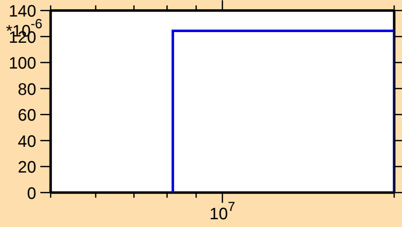
\sigma vs. E for ^{219}\text{Rn}(n,d)
