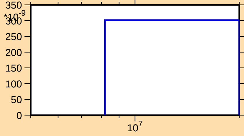
\sigma vs. E for ^{219}\text{Rn}(n,nt)
