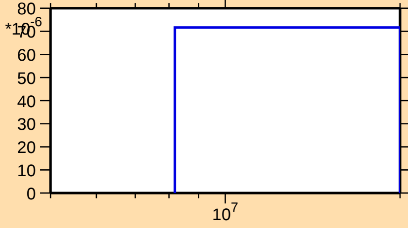
\sigma vs. E for ^{219}\text{Rn}(n,np)
