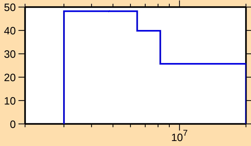
\Delta\sigma/\sigma vs. E for ^{219}\text{Rn}(n,2n)
