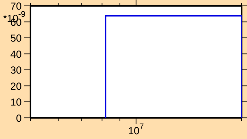
\sigma vs. E for ^{219}\text{Rn}(n,2np)
