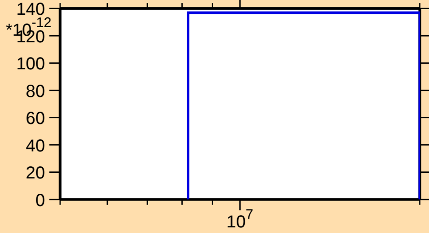
\sigma vs. E for ^{219}\text{Rn}(\text{mt117})
