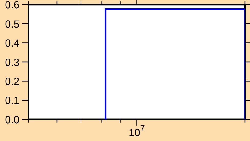
\sigma vs. E for ^{219}\text{Rn}(n,3n)
